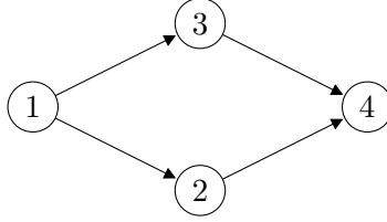
Figure 1: Graph for Example 2.3 and the proofs of Propositions 3.1, 4.3, and 4.4.
