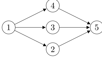
Figure 3: Graph for the proof of Proposition 3.7.
