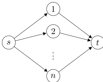
Figure 4: Network for the proof of Proposition 3.8.
