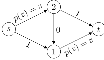
Figure 5: Network and price functions for Example 3.11.
