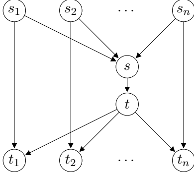
Figure 2: Network for the proof of Proposition 3.5.
