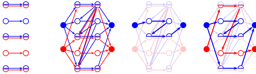
Figure 2: Vehicle scheduling in a small example. From left to right: trips; depots, trips and all legal connections; a rotation; a schedule.
