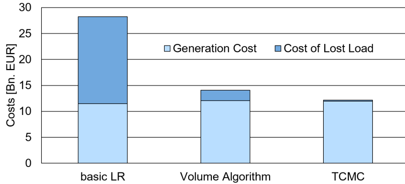
Figure 5: Comparison of Generation and Loss-of-Load costs in the German market area
