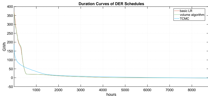
Figure 3: Duration curves of DER schedules
