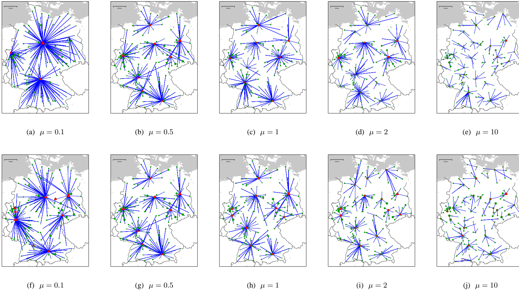
Figure 8. Result for MSC location planning. Upper row 3.4 million users, lower row 6.8 million users
