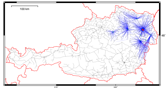
Figure 12. Solution for regions Vienna, Burgenland, and Lower Austria
