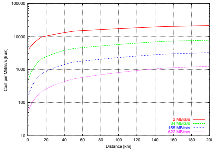
Figure 1. Cost rel. to distance per Mbit/s
