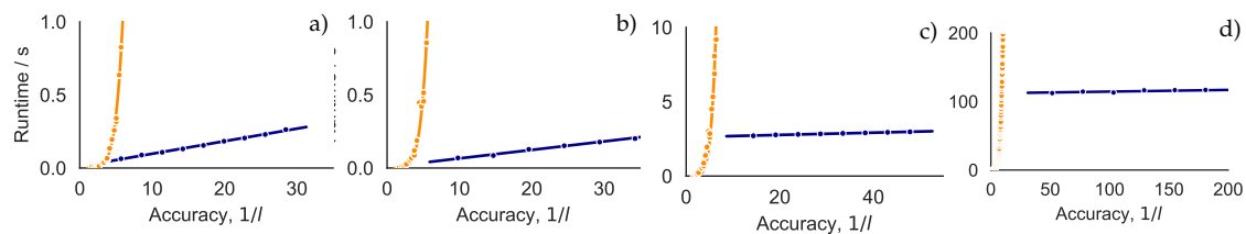
Figure 9: Minimum runtime in seconds taken experiments similar to Fig. 8. Blue: DisCOptER Algorithm with l_c := \delta\tau L , linear trend line. Orange: Purely discrete, polynomial trend line of order 6.
