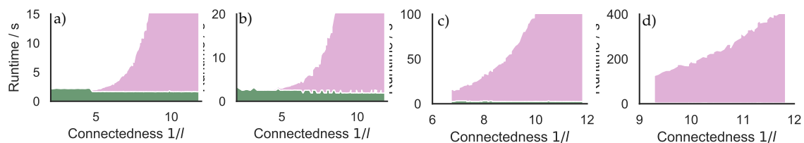
Figure 8: Runtimes of the DisCOptER algorithm in seconds, split into the discrete part (pink, top) and the continuous part (green, bottom), sampled with h = l^2 . Constant accuracy \delta\tau = 1/300 .
