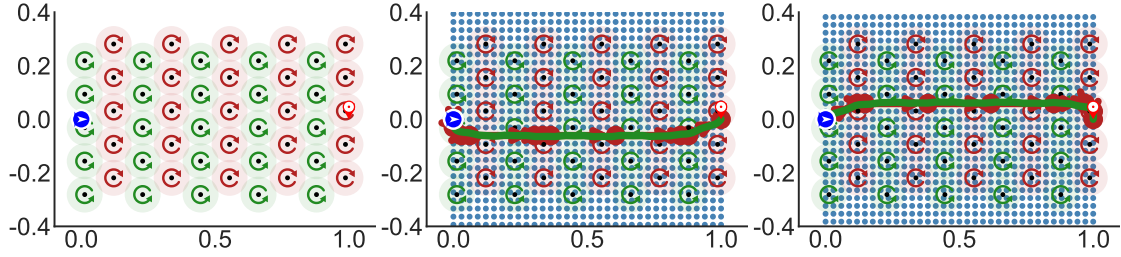
Figure 5: Test problem d) with 50 vortices (10 columns of 5 vortices each), R = 1/16 , regularly positioned. x_O = [0, 0]^T , x_D = [1, 0]^T , \bar{w} = 0.5\bar{v} . Blue dots: graph with h = l^2 and 1/h_x = 33 and 34, respectively, Red: discrete optimal trajectory, Green: continuous optimal trajectory. Note that, again, the straight trajectory is particularly unfavorable. This problem is point-symmetric w.r.t. [0.5, 0]^T . The two shown solutions are equivalent.
