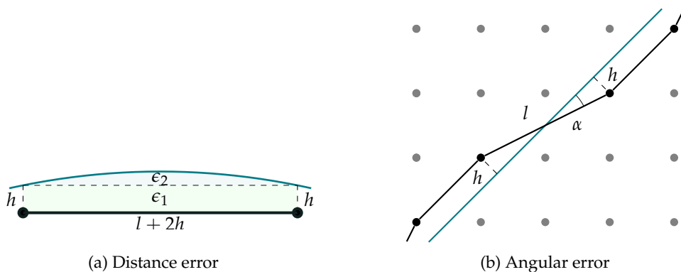
Figure 1: Geometrical error bounds. Blue line: continuous optimal solution. Black line: discrete optimal solution. Gray dots: graph nodes.
