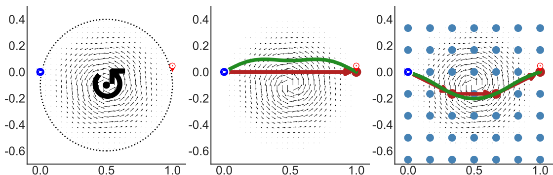
Figure 3: Test problem b) with counterclockwise spinning vortex centered at z = [0.5, -0.1]^T , R = 0.5 . x_O = [0, 0]^T , x_D = [1, 0]^T , \bar{w} = \frac{1}{2}\bar{v} . Blue dots: network graph with h = l^2 and 1/h_x = 1 and 6, respectively, Red: discrete optimal trajectory, Green: continuous optimal trajectory.
