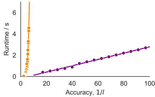
Figure 6: Test case a). Orange: Discrete-only approach, polynomial trend line of order 6. Purple: Newton-KKT initialized with straight line, l \doteq l_C = \delta\tau L , linear trend line.
