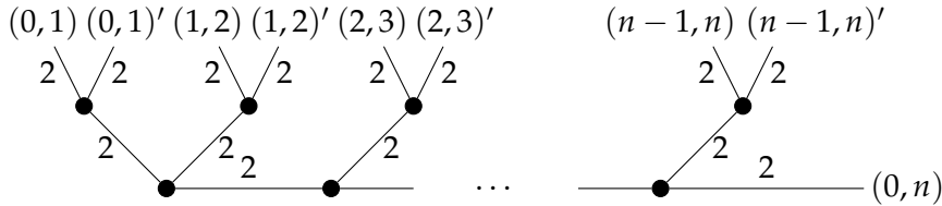
Figure 3: An optimal branch decomposition of width 2 for the I(r, c, C) network
