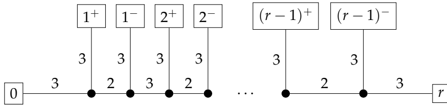
Figure 4: An optimal carving decomposition of width 3 of the modified I(r, c, C) network
