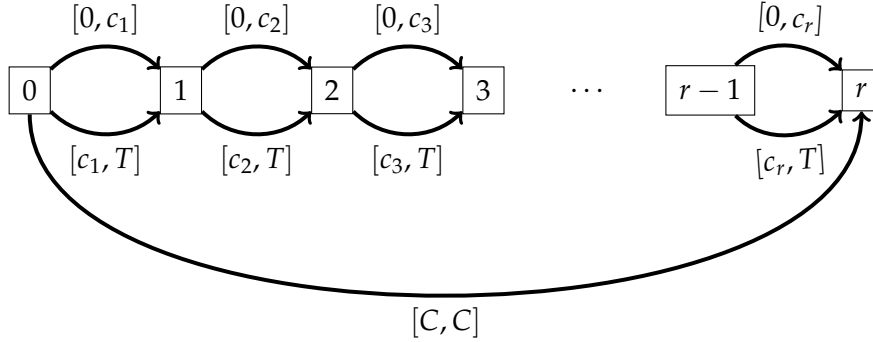
Figure 1: Instance I(r, c, C) : arcs a are labeled with [\ell_a, u_a] , T := \sum_{i=1}^r c_i + 1
