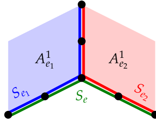
Figure 5: Relation between S_e, S_{e_1} and S_{e_2}
