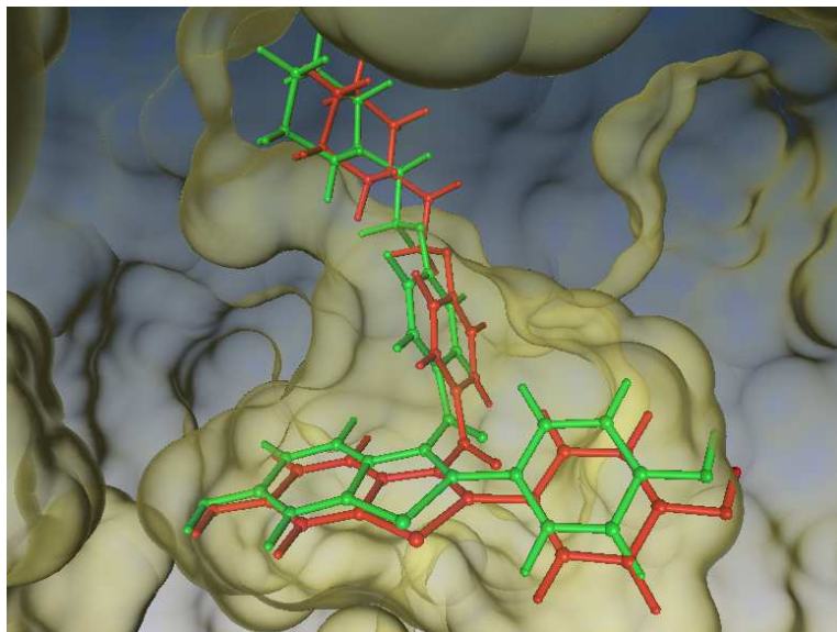
Figure 6: Estrogen receptor depicted in molecular surface representation (transparent), antagonist as contained in 1err in ball and stick representation. Experimentally resolved binding mode mapped in green, docked binding mode after Fine-Tuning in red.
