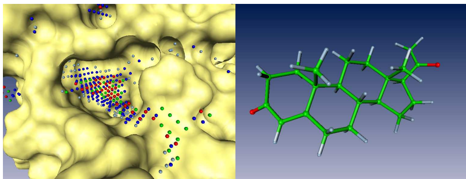
Figure 7: Left: Pharma site of the anti-steroid antibody together with molecular surface. Attentive observation reveals the grid structure of the pharma site. Right: Progesterone featuring two carbonyl oxygen atoms.
