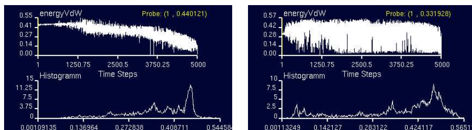
Figure 3: Left: Trajectory containing 5000 Point-Matching solutions for CDK 2 sorted by RMSD from crystal coordinates starting from the smallest value. In the upper graph the individual time-steps are plotted against the scoring energy. Right: Same for the estrogen receptor
