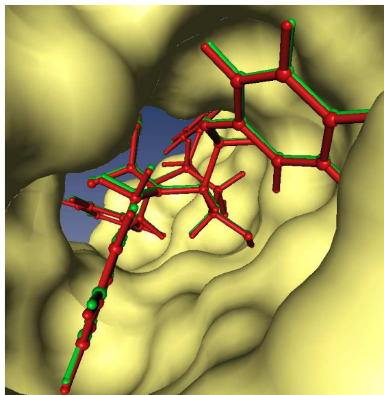
Figure 5: HIV1-protease depicted in molecular surface representation, inhibitors in ball and stick representation. Experimentally resolved binding mode mapped in green, docked binding mode after Fine-Tuning in red (RMSD:0.22Å).
