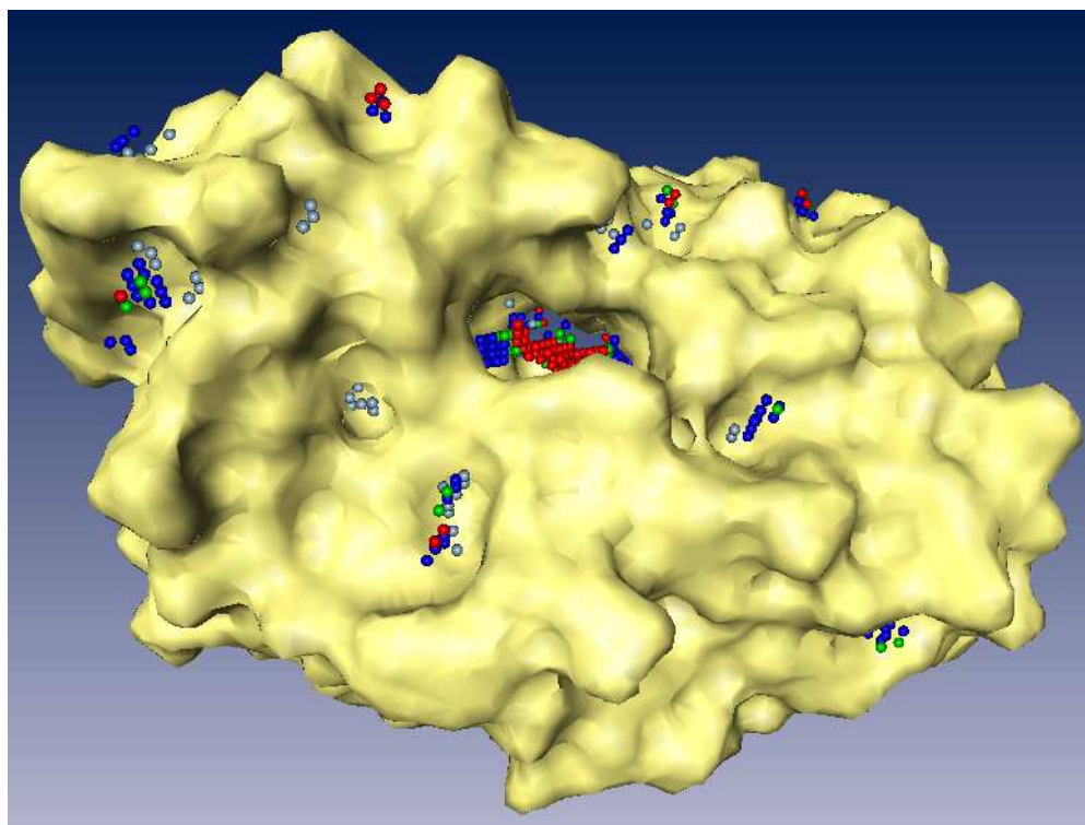
Figure 2: HIV-1-protease in molecular surface view together with its pharma site. Donors in grey, acceptors in red, aromatics in green and aromatic acceptors in blue.
