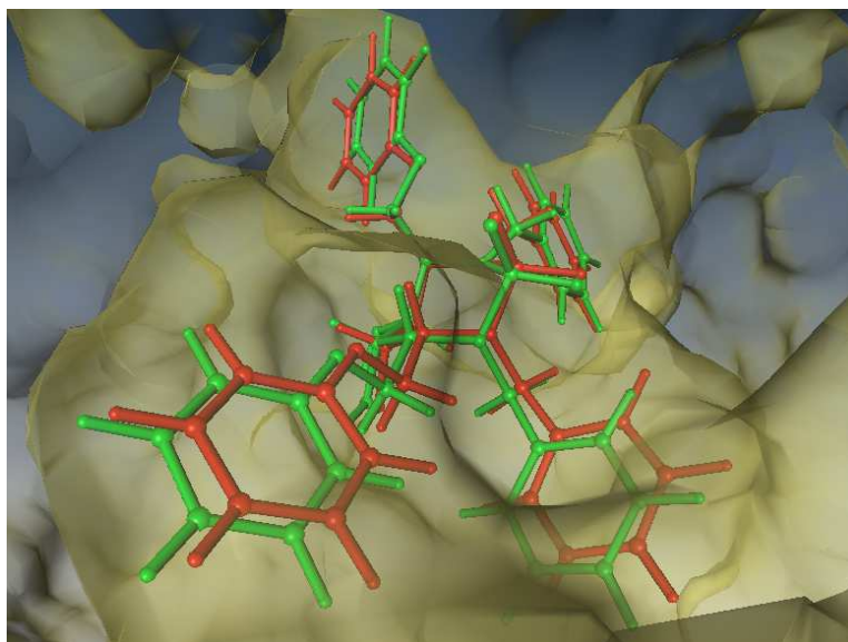
Figure 4: HIV-1-protease depicted in molecular surface representation, HIV-1-protease Inhibitors in ball and stick representation. Experimentally resolved binding mode mapped in green, binding mode according to Point-Matching in red (RMSD:0.77Å).
