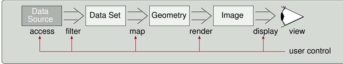
FIG. 3.1. Most visualization systems share the same underlying visualization pipeline [9]. The components of the pipeline can be freely distributed, in principle, as the communication elements between these components have different demands on latency and bandwidth required. All elements of the pipeline should be controlled by the end user or by the application.
