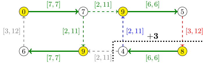
Figure 1: Fundamental delay cut: In this PESP instance with T = 10 and w \equiv 1 , delaying the two vertices at the right lower corner by 3 produces a better (in fact, optimal) timetable: The overall slack is reduced from 7 to 4. This corresponds to the fundamental cut of the green spanning tree when removing the red arc. The modulo network simplex inner loop replaces the red arc with the blue arc at its lower bound.
