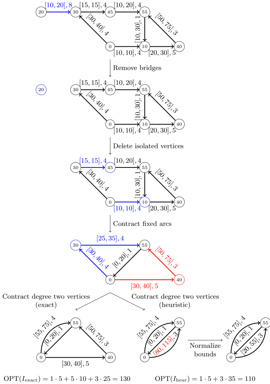
Figure 3: Exact and heuristic preprocessing
