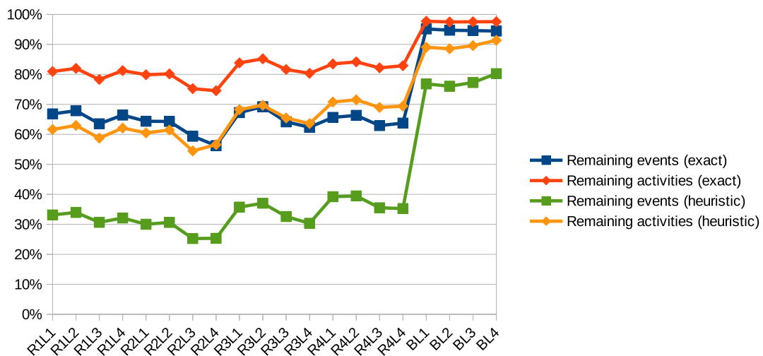
Figure 8: Size reduction by preprocessing
