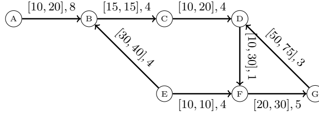
Figure 5: The PESP instance from Example 1 with named events, T = 60 .
