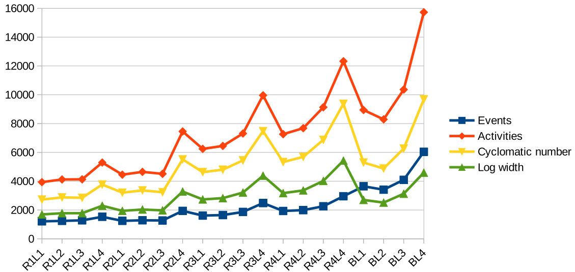
Figure 7: Sizes of PESplib instances after heuristic preprocessing
