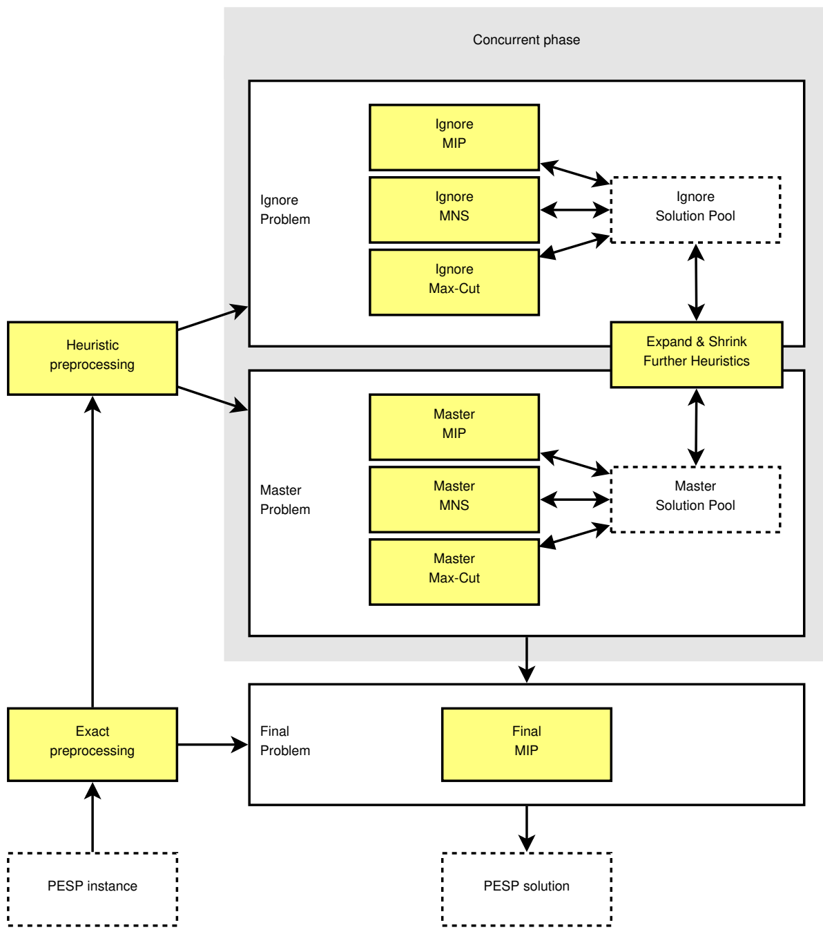
Figure 2: Architecture of our concurrent PESP solver
