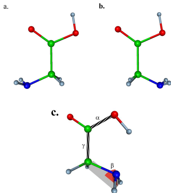
Figure 4: Mean molecules calculated from 3 metastable subsets of the uncharged form of the amino acid glycine: The thermodynamical weights of conformation a,b,c at 300K are 0.48%, 0.29%, 99.23%
