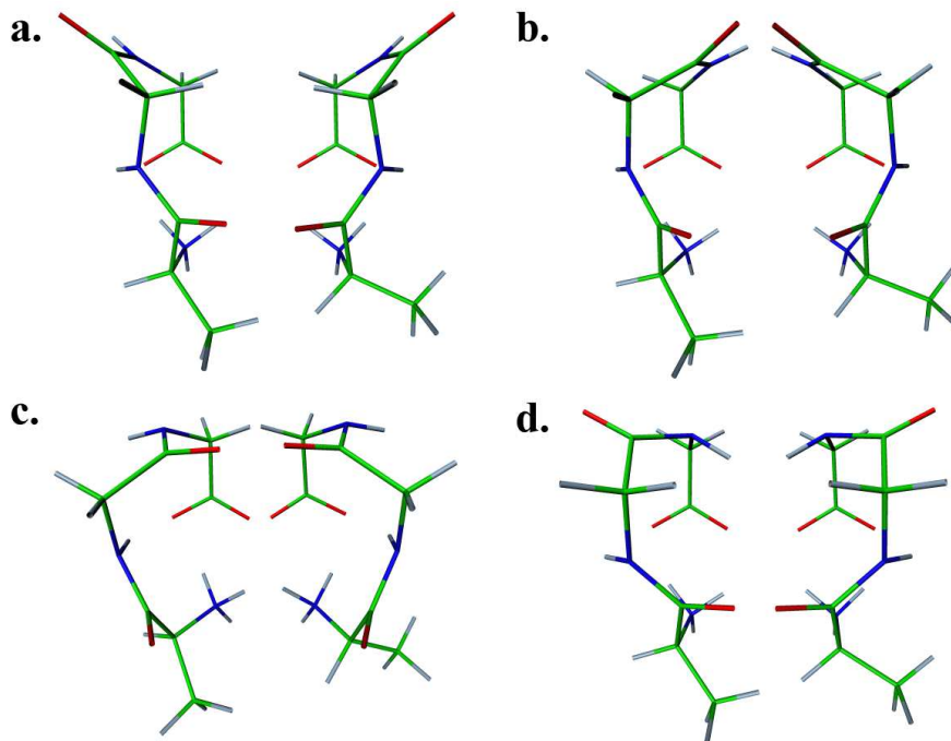
Figure 5: Mean molecules calculated from 8 metastable subsets of the peptide ala-gly-gly: The molecules are arranged in pairs to emphasize the partial symmetry of the conformations. The thermodynamical weights of the conformations in a,b,c, and d at 300K are 63.07% and 33.18%, 1.52% and 1.66%, 0.19% and 0.08%, 0.09% and 0.05%
