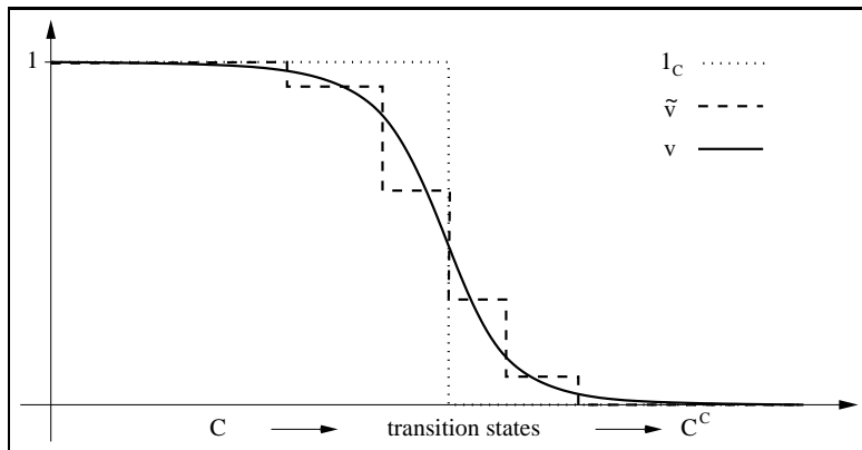
Figure 1: Transition region between metastable conformations: Characteristic \mathbb{1}_C versus membership function v and discretization \tilde{v} of v .
