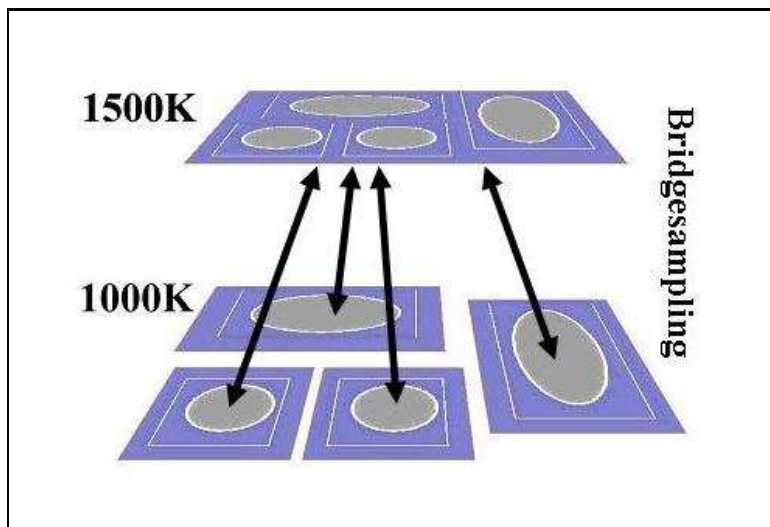
Figure 3: Hierarchical simulation protocol: After decomposition, the metastable subsets of the conformational space are sampled independently at a lower temperature level. Two temperature level are connected via bridge sampling, i.e. the HMC simulation samples a generalized distribution, which is constructed from the canonical distributions of both temperatures [7].
