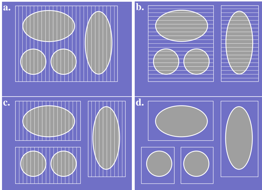
Figure 2: Algorithmic scheme for successive PCCA of dihedrals: Four metastable regions are drawn as ellipses in a 2-dimensional dihedral space. Thin lines show the fine discretization of the dihedral, which indicates highest metastability according to the second eigenvalue of the corresponding transition matrix. Figures a. to d. illustrate the alternation of fine discretization followed by coarse decomposition.
