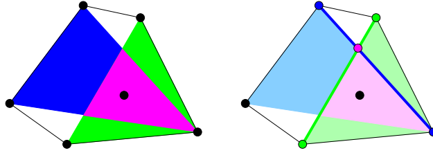
FIGURE 2. An unwanted intersection can be detected by a circuit
