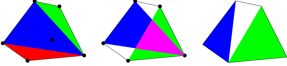
FIGURE 1. A correct triangulation, an unwanted intersection (IP not met), and an incomplete triangulation (UP not met)
