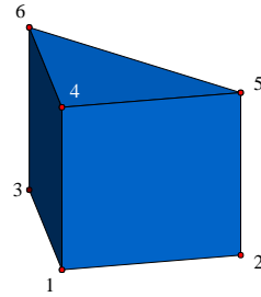
FIGURE 10. Convex lifting function and regular subdivision [Rei]
