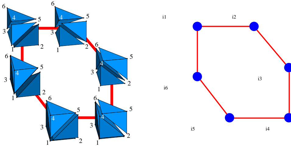
FIGURE 12. How to construct geometrically the six initial ideals of the unimodular ideal I_{\mathcal{A}} = \langle \partial_1\partial_5 - \partial_2\partial_4, \partial_1\partial_6 - \partial_3\partial_4, \partial_3\partial_5 - \partial_2\partial_6 \rangle : The generators of each initial ideal are precisely the minimal non-faces of the corresponding regular triangulation of \mathcal{A} .
