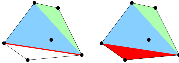
FIGURE 3. An interior facet covered by only one simplex detects a (UP)-violation; another simplex containing it is required
