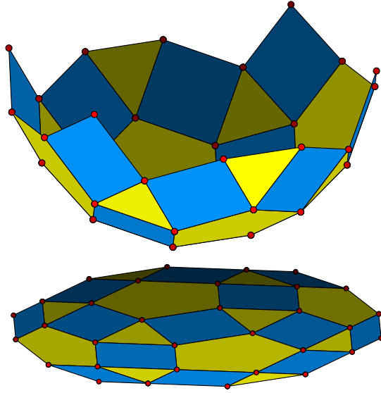
FIGURE 10. Convex lifting function and regular subdivision [Rei]
