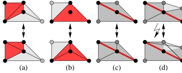
FIGURE 9. All possible flip types in dimension two; the rightmost picture shows a situation where the links of all maximal simplices are not equal, whence the corresponding flip is impossible
