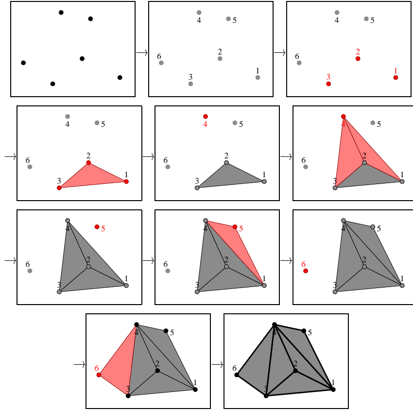
FIGURE 7. Constructing a placing triangulation
