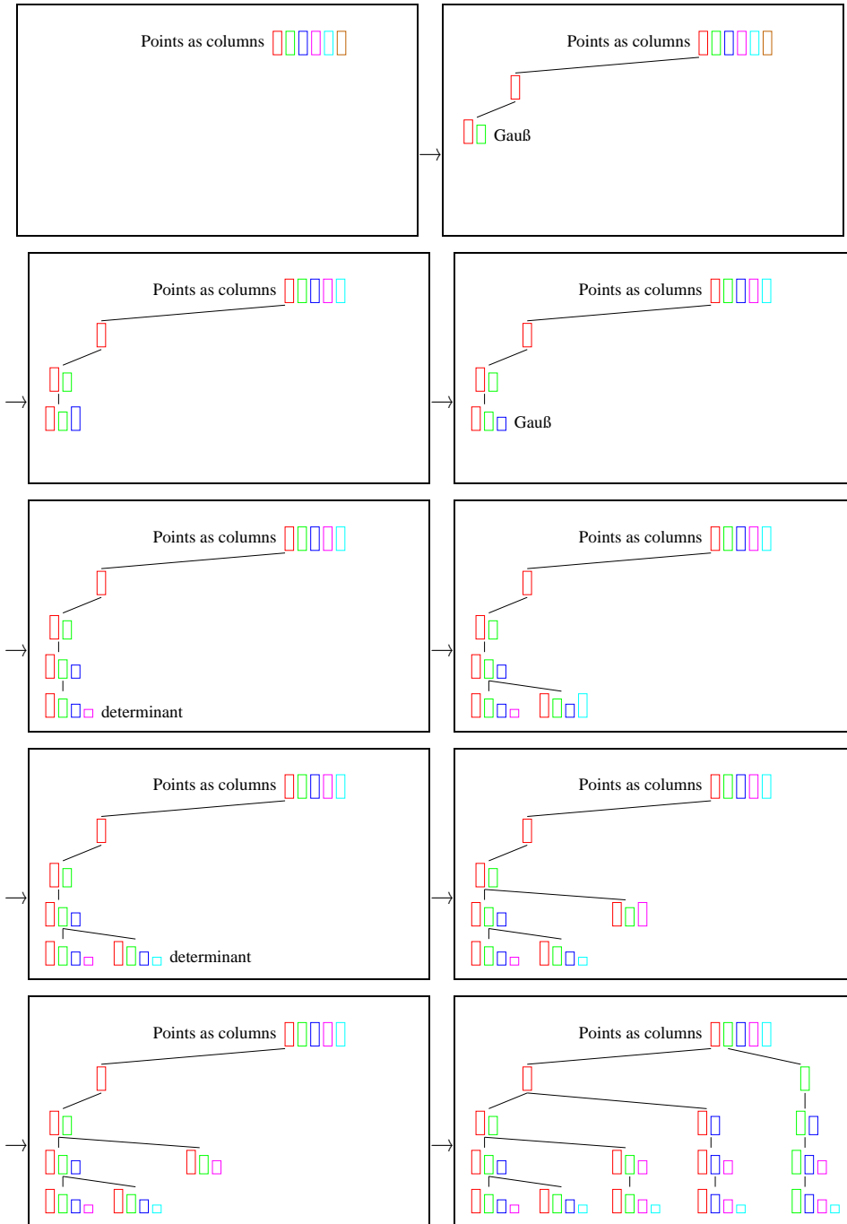
FIGURE 5. Building the computation tree for the chirotope: the matrices in the nodes are all transformed in column normal form before new columns are added (indicated are regions of possible non-zeroes in the columns); the determinants can be computed easily at the leaves
