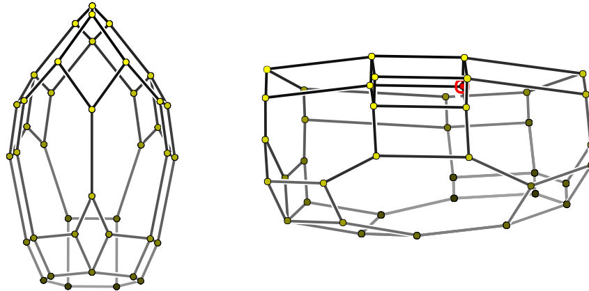
FIGURE 13. Left: Secondary polytope of the cyclic 4-polytope with 8 vertices. All 40 triangulations are regular. Right: Secondary of a different neighborly 4-polytope with 8 vertices [Grü67, Ch. 7], which has one nonregular triangulation (circled; in the interior of the convex hull) among 41
