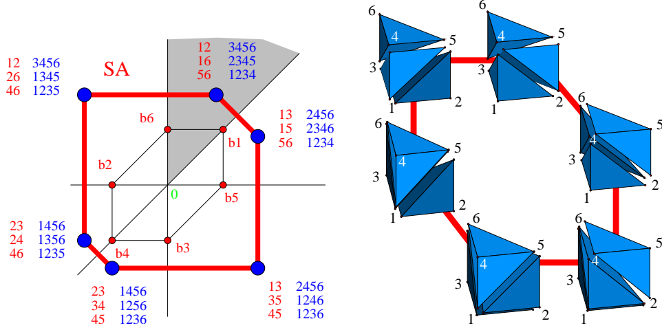
FIGURE 11. The hexagon as the secondary polytope of the prism P . Left : One maximal cone of the secondary fan is highlighted. Pairs of digests inside such a cone \sigma index vertices b_i in whose positive span \sigma lies, and the complementary 4-tuples label the simplex of the triangulation of \mathcal{A} that \sigma corresponds to. Right : Triangulations corresponding to vertices of \Sigma(P) . Edges of \Sigma(P) representing flips between triangulations.
