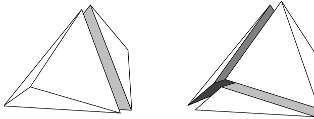
FIGURE 8. The two possible triangulations of five points in general position in dimension three; Z^- contains, w.l.o.g., the three vertices of the interior cutting face in the left picture; Z^+ contains the two vertices of the interior cutting edge in the right picture
