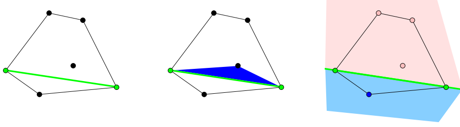
FIGURE 4. A facet F in T , i.e., a facet of some simplex in T , is interior if the cocircuit of \mathcal{A} spanned by F has both positive and negative elements
