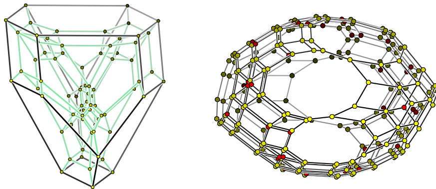
FIGURE 14. Left: Schlegel diagram of the secondary polytope of the 3-cube [P00a]. All 74 triangulations are regular. Right: Secondary of the cyclic 8-polytope with 12 vertices, realized on the Carathéodory curve [P00b]. There are 42 nonregular triangulations among 244 in all
