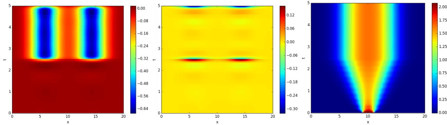
Figure 1: Computed optimal control (left), difference to exact control (middle) and optimal state (right) using IMEX.
