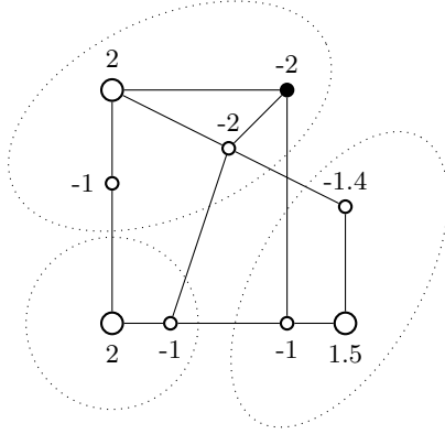
Figure 1: A positive-vertex decomposition of an MWCSF instance with regions marked by dotted ellipses. Lemma 1 guarantees that the (upper right) filled vertex can be deleted if a lower bound higher than U_2 = 2.5 is given.
