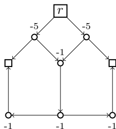
Figure 4: Illustration of a directed RMWCSP instance with vertices R drawn as squares. The Cut_r formulation yields an optimal LP solution with objective value -7.5 , while TransCut_{FB} leads to an optimal LP solution with objective value -8
