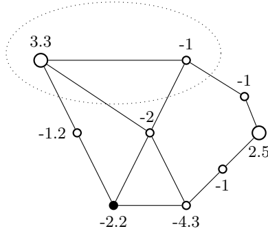
Figure 2: An MWCSP instance. Considering the vertices marked by the dotted ellipse as the set W , one can verify with Lemma 9 that the (bottom left) filled vertex can be deleted.
