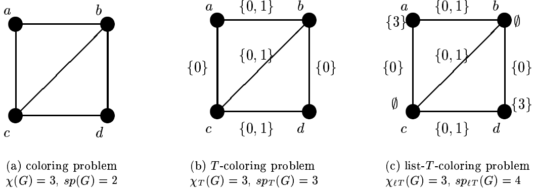
Figure 2: Example coloring, T -coloring, list- T -coloring.
