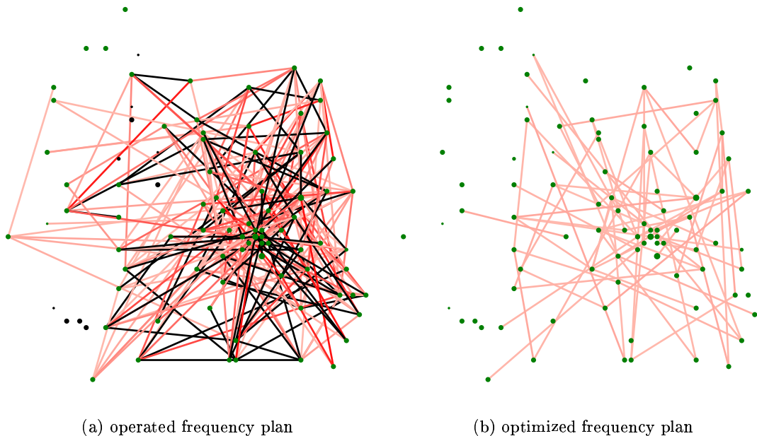
Figure 5: Interference reduction of 96% by heuristics.
