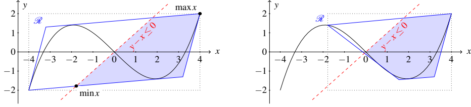
Figure 3: Example \min\{y - x : y = 0.1x^3 - 1.1x, x \in [-4, 4], y \in [-2, 2]\} . On the left, the shaded region over which OBBT is performed is defined by the LP relaxation \mathcal{R} and the dashed objective cutoff resulting from the zero solution. Minimizing x gives a lower bound of -\frac{16}{9} and the LVB x \geq -\frac{10}{9}U - \frac{16}{9} . Maximizing x does not tighten its upper bound, still the LVB x \leq \frac{10}{37}y + \frac{128}{37} can be learnt. In this two variable example, this is only the rightmost facet of \mathcal{R} , but in higher dimensions it may be nontrivial. On the right is the resulting, tighter relaxation.
