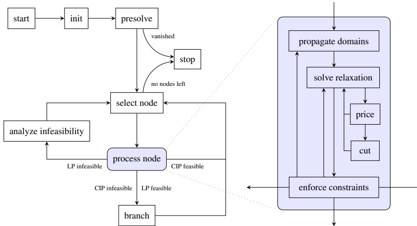
Figure 1: Flowchart of the main solving loop of SCIP.
