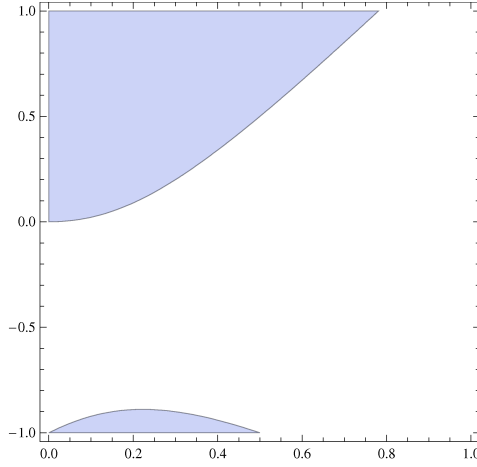
Figure 2: Feasible region of inequality (11).
