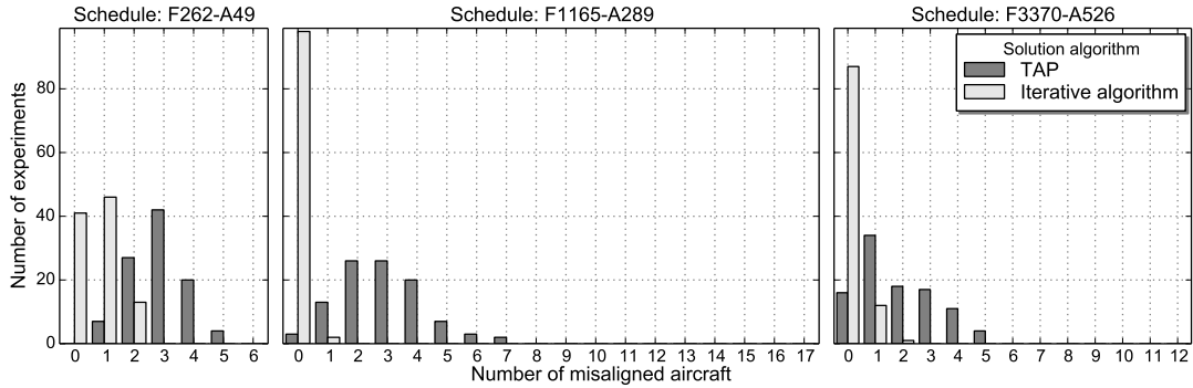
Figure 6: Comparing the TAP and iterative algorithm with histograms of the number of maintenance misaligned aircraft at the end of day-one over a set of 100 experiments using the SDAMRP LOF.
