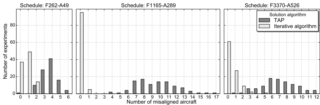
Figure 5: Comparing the TAP and iterative algorithm with histograms of the number of maintenance misaligned aircraft at the end of day-one over a set of 100 experiments using the aircraft routing LOF.
