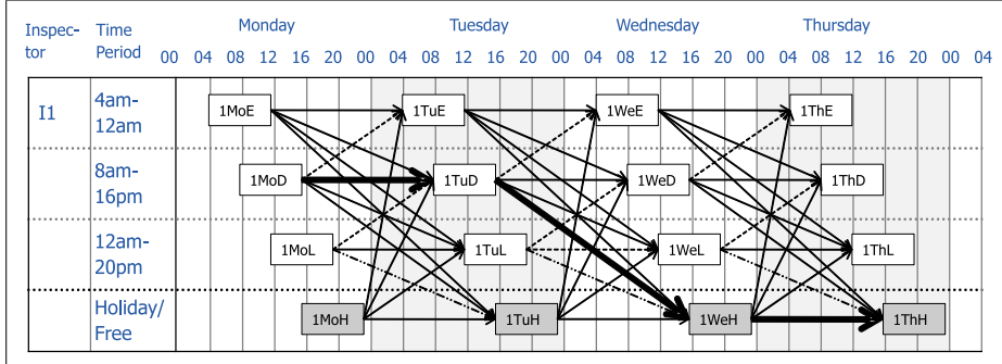
Figure 2: Excerpt of an Inspector Roster Graph with one inspector, three time periods and four days.
