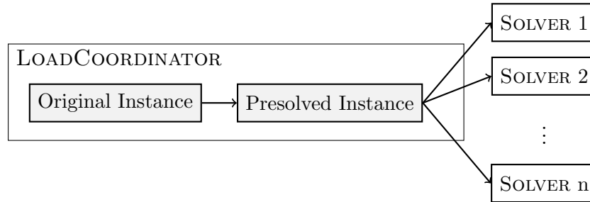
Figure 1: Initialization step
