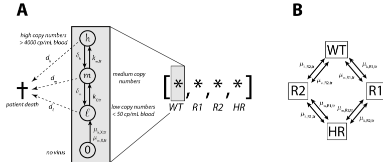
Figure 2: Simplified HIV Model A: Transitions between copy number states n_C . B: Transitions in between viral strains M .
