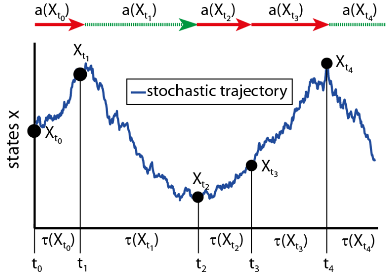
Figure 1: Schematic illustration of the presented control model. The graphic highlights that the examination times t_j and sequence of actions are random variables because the underlying process is a random realization: The solid blue line indicates the disease process within an individual patient (a stochastic realization of the process), while the solid black dots indicate the examination times t_j for this particular stochastic realization, which depend on the observed state from the last examination time and the stationary deterministic decision rule.
