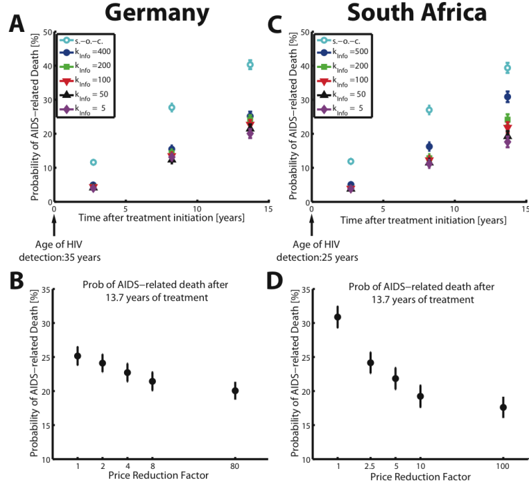
Figure 3: Effect of resistance test k_{\text{info}} cost reduction on AIDS survival A: Probability of AIDS-related death 1000-, 3000- and 5000 days after treatment initiation under application of a standard-of-care treatment (open cyan circles) vs. a cost-optimal policy with drug resistance test costs k_{\text{info}} = 400, 200, 100, 50, 5 US$ per test (blue dots, green squares, red downward-pointing triangles, black upward-pointing triangles and magenta diamonds) in a resource-rich setting (Germany). B: Probability of AIDS-related death 5000 days after treatment initiation as a function of resistance test price reduction in a resource-rich setting (Germany). C: Probability of AIDS-related death 1000-, 3000- and 5000 days after treatment initiation under application of a standard-of-care treatment (open cyan circles) vs. a cost-optimal policy with drug resistance test costs k_{\text{info}} = 500, 200, 100, 50, 5 US$ per test (blue dots, green squares, red downward-pointing triangles, black upward-pointing triangles and magenta diamonds) in a resource-constrained setting (South Africa). D: Probability of AIDS-related death 5000 days after treatment initiation as a function of resistance test price reduction in a resource-constrained setting (South Africa).
