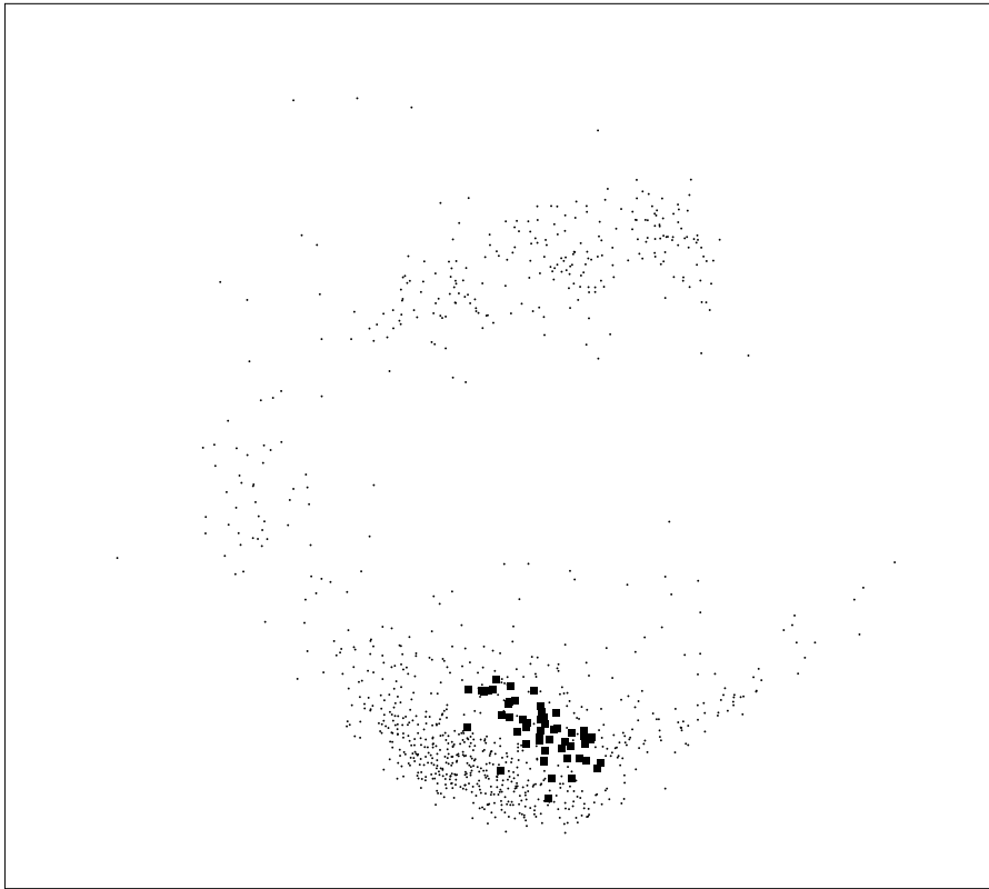
Figure 1: Two-dimensional map of 1000 configurations chosen from a molecular dynamics trajectory
