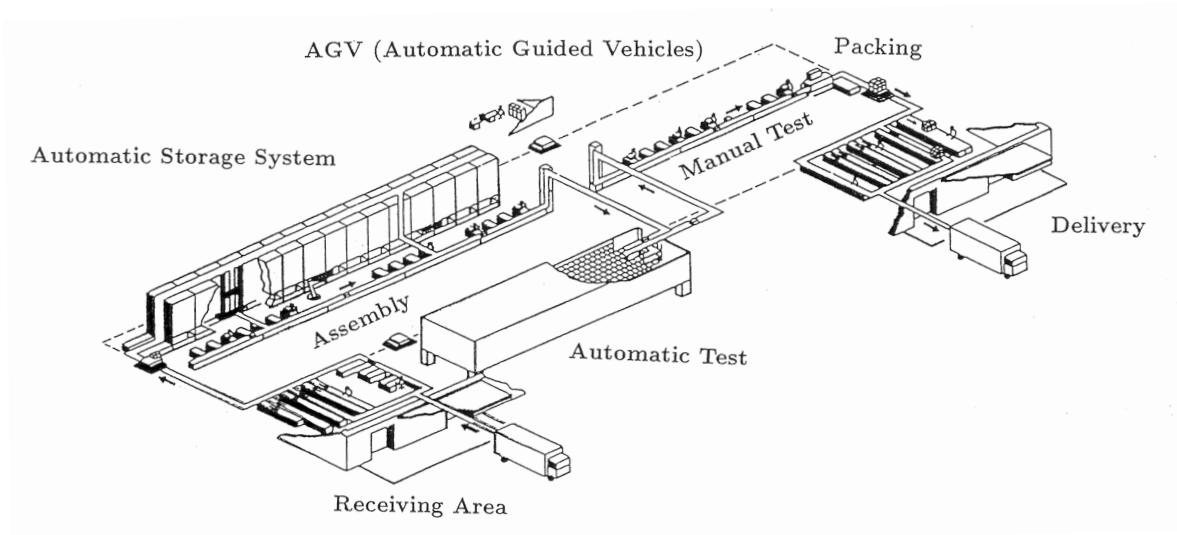
Figure 1.1 Sketch of the factory layout
