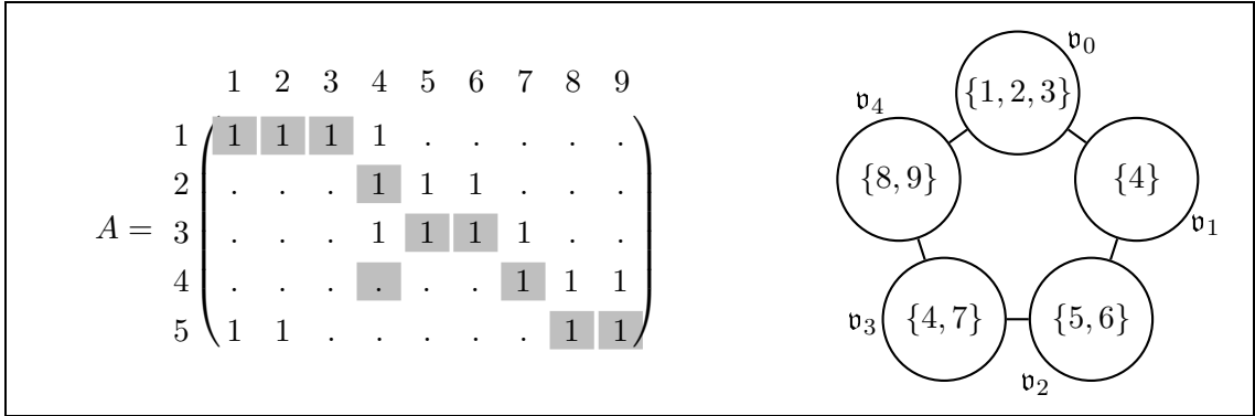
Figure 4: A Not Sekiguchi Partitionable 0/1 Matrix and a 5-Cycle of Columns.
