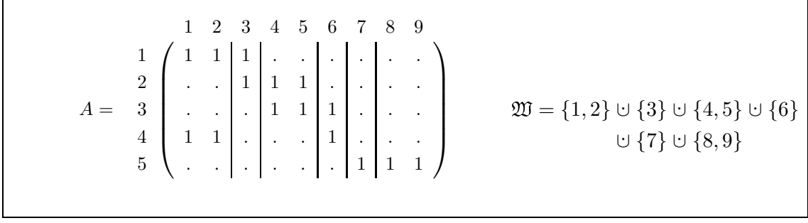
Figure 3: A Sekiguchi Partitionable 0/1 Matrix.
