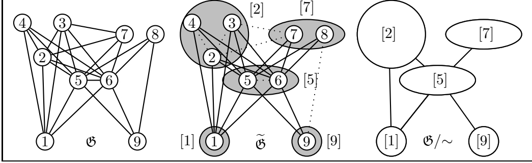
Figure 2: Constructing a Class Conflict Set Packing Relaxation.
