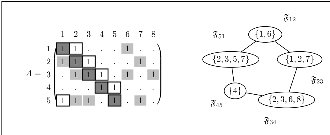
Figure 5: A 5-Cycle of (i, j) -Families.
