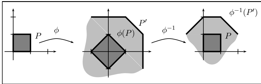
Figure 1: Constructing a Combinatorial Relaxation.
