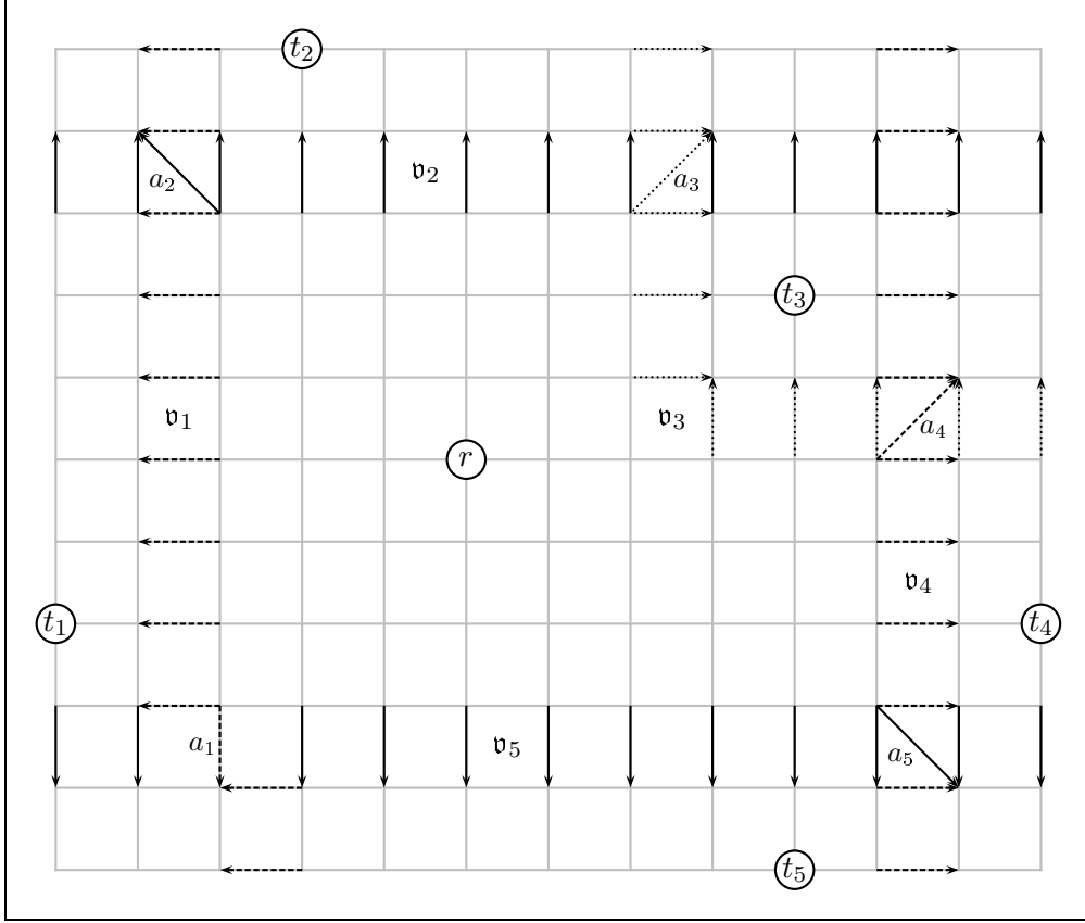
Figure 6: A 5-Cycle of Steiner Protocols in a Planar Grid Digraph.
