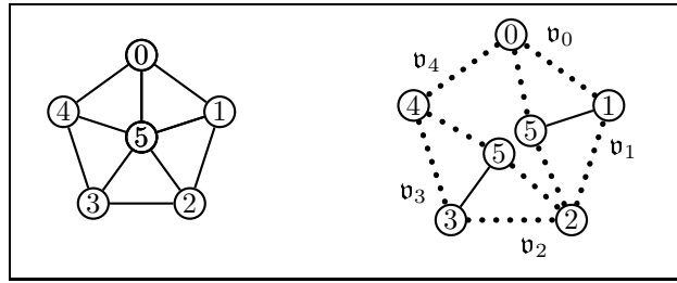
Figure 9: A Cycle of Nodes and Edges.
