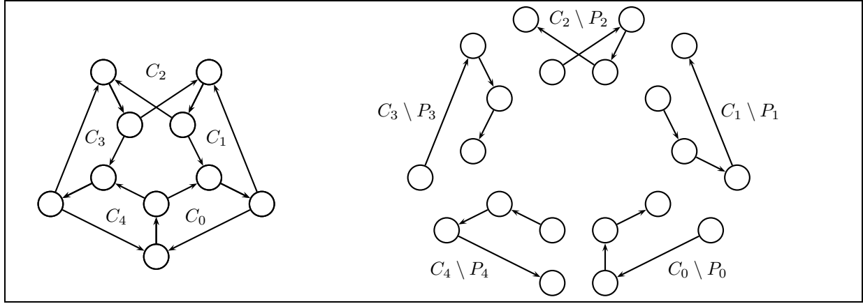
Figure 4: A Möbius Cycle of Dipaths.
