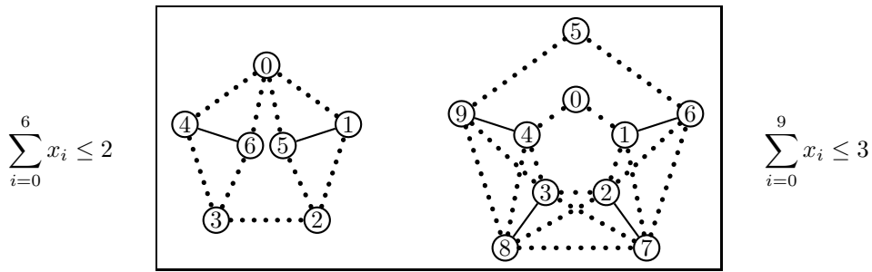
Figure 10: Two Generalizations of Odd Wheel Inequalities.
