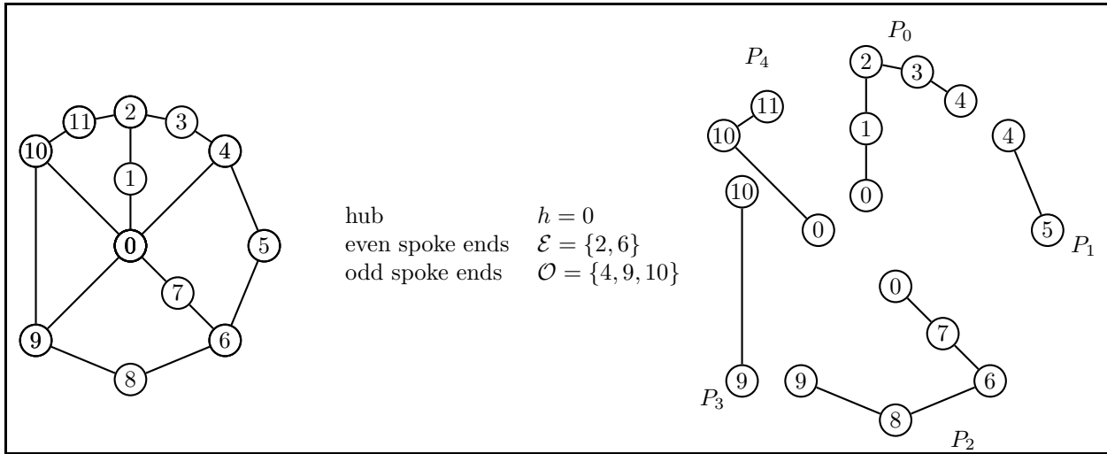
Figure 12: A 5-Wheel and a 5-Cycle of Paths of Type II.
