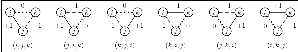
Figure 6: Labeling Lower Triangles.
