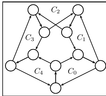
Figure 2: A Möbius Ladder of 5 Dicycles.
