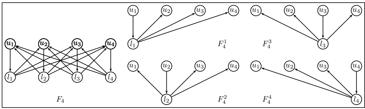
Figure 3: A Fence Clique of Forks.
