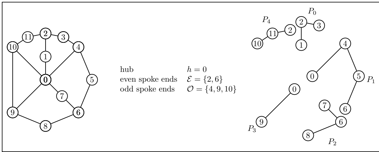
Figure 11: A 5-Wheel and a 5-Cycle of Paths of Type I.
