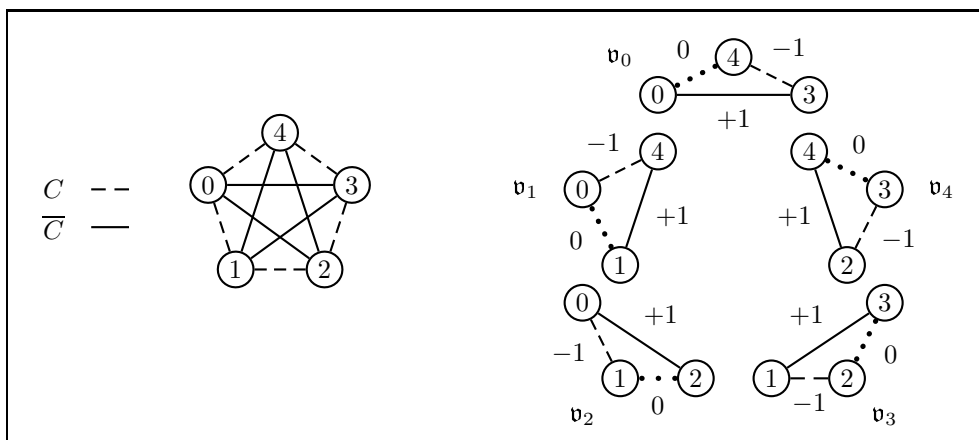
Figure 7: An Odd Cycle of Lower Triangle Inequalities.
