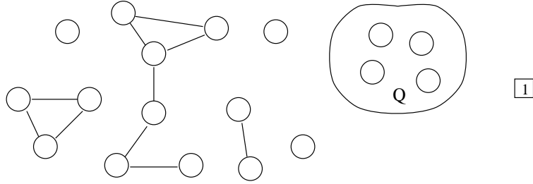
Figure 3.1 The feasibility graph G_F (with node 1 added)
