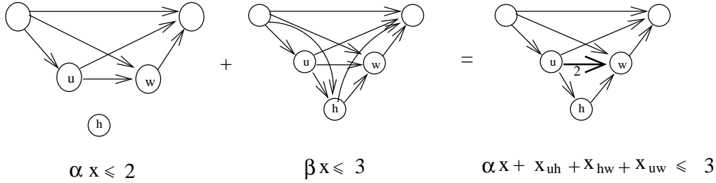
Figure 4.7 V-lifted tournament constraint
