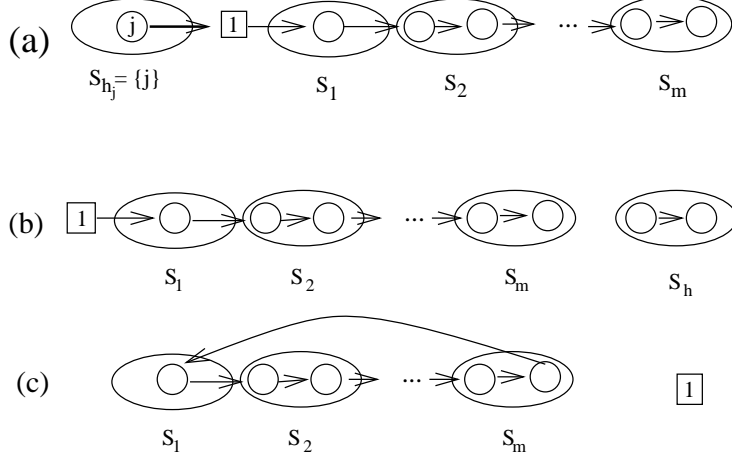
Figure 3.3 Constructions for the proof of Lemma 3.5
