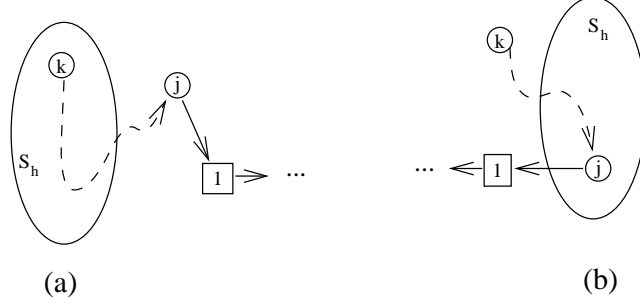
Figure 3.2 Illustration for the proof of Lemma 3.4
