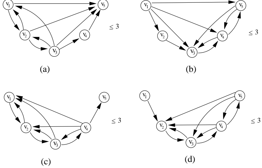
Figure 4.6 Lifted infeasible path constraints on k = 5 nodes
