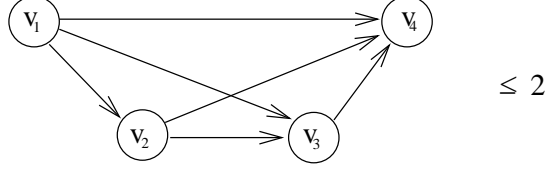
Figure 4.4 The support graph of a tournament constraint on k = 4 nodes
