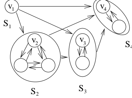
Figure 4.5 A generalized tournament constraint
