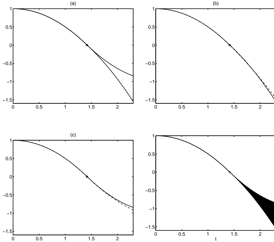
Figure 1: Illustration ( q^1 vs. t ) of the sensitivity on \mu and \epsilon , indicating Takens-chaos: (a) the two different limit solutions q_0^{\mu=0} and q_0^{\mu \downarrow 0} , (b) the limit solution q_0^{\mu=0} (solid line) and the QCMD-solution for \epsilon = 0.05 and \mu = 0.1 (dashed line), (c) the limit solution for \epsilon \rightarrow 0 with \mu = 0.1 (solid line) and the QCMD-solution for \epsilon = 0.005 and \mu = 0.1 (dashed line), (d) the funnel of possible limits for \epsilon \rightarrow 0 , \mu \rightarrow 0 .
