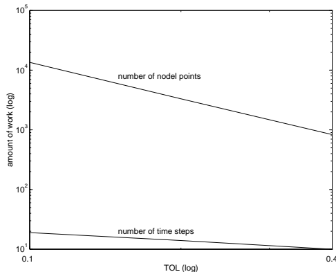
Figure 1: Number of Time-Steps and Nodal Points vs. Tolerance TOL (Example 1)
