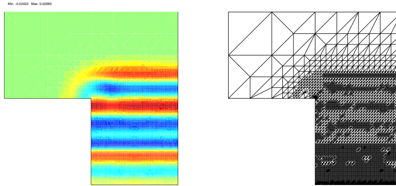
Figure 3: Solution and Triangulation for Time-Step # 20 (Example 2)
