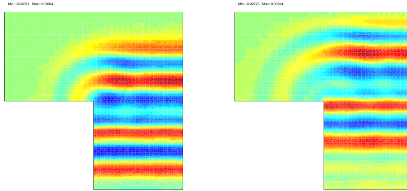
Figure 4: Solution for Time-Step # 30 and # 40(Example 2)
