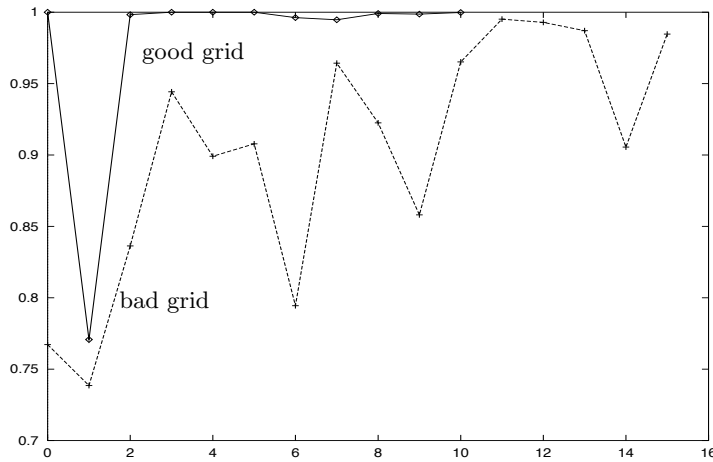
Figure 5: Iterative damping factors [\bar{\lambda}_k] for “good” and “bad” initial coarse grids ( standard mesh refinement option).
