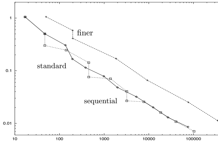
Figure 4: Iterative (exact) energy error norms \epsilon_k^{1/2} versus number of nodes N_k for three mesh refinement options.
