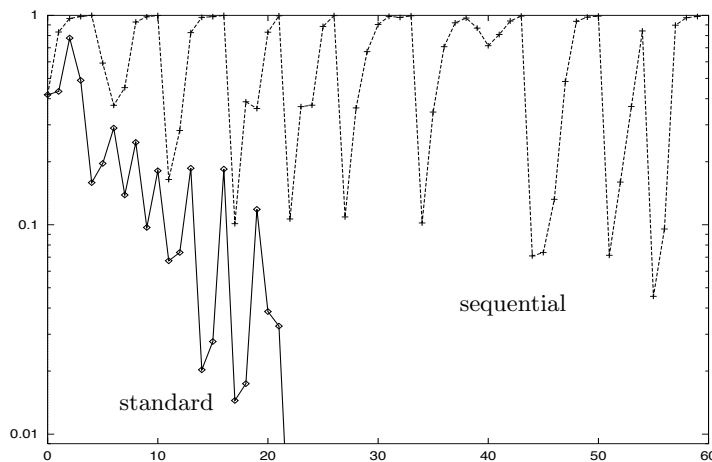
Figure 6: Standard versus sequential mesh refinement option in terms of damping factors \lambda .
