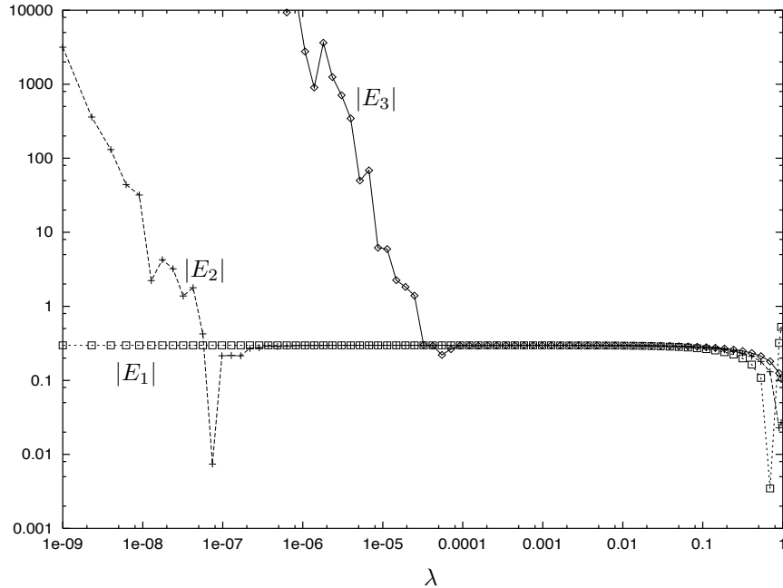
Figure 1: Cancellation of leading digits in estimators [h_k] based on formulas for |E_3| , |E_2| , |E_1| , respectively.
