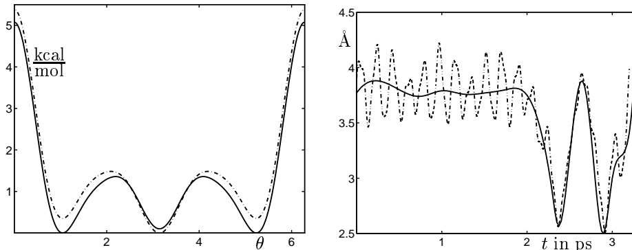
Figure 3: Left hand side: Torsion angle potential V_{tor} (dashed line) and the corrected potential V_{tor} + W for the scenario explained in the text (solid line) in kcal/mol versus the torsion angle \theta . In the corrected potential the minimum at \theta = \pi is no longer the global minimum. Right hand side: Evolution of the distance |q_1 - q_4| with t for the original MD-solution (dashed line) and for the limit solution (solid line) for the scenario explained in the text.
