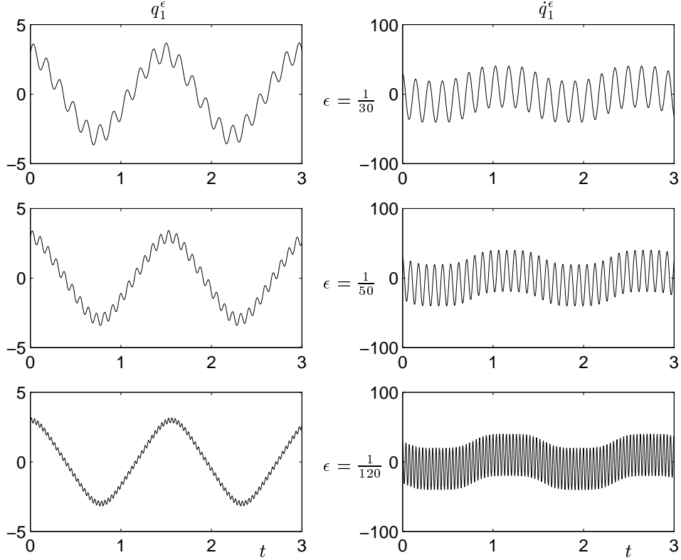
Figure 1: Illustration of the convergence with \epsilon \rightarrow 0 for the system (3.4) in the two-dimensional collinear case with V(q) = q_1^4 and U(q) = (q_2 - q_1)^2/2 : on the left hand side the first component q_1^\epsilon of the solution versus time for \epsilon decreasing from top to bottom ( \epsilon = 1/30, 1/50, 1/120 ), on the right hand side the corresponding derivatives \dot{q}_1^\epsilon in the corresponding order. The total energy is identical in all three cases. Note that q_1^\epsilon converges strongly to its running average while \dot{q}_1^\epsilon converges only weakly.
