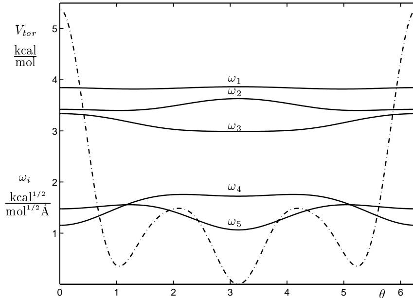
Figure 2: Dashed line: Torsion angle potential V_{tor} versus torsion angle \theta . Note that the potential is symmetric with respect to the main minimum located at \theta = \pi with two equal local minima near \theta = \pi/3, 5\pi/3 . Solid lines: Frequencies \omega_i of the fast oscillations normal to \mathcal{M} versus the torsion angle \theta . Note the crossings of the two lowest frequencies near the local minima of V_{tor} . They are connected to resonances of the fast oscillations.
