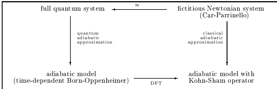
Figure 1: Logic of the Car-Parrinello method
