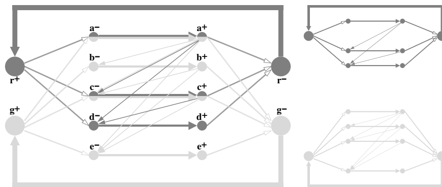
Abb. 2. Digraphen (V, A) und (V_d, A_d) zu \mathcal{D} = \{r, g\} , \mathcal{T} = \{a, b, c, d, e\} .
