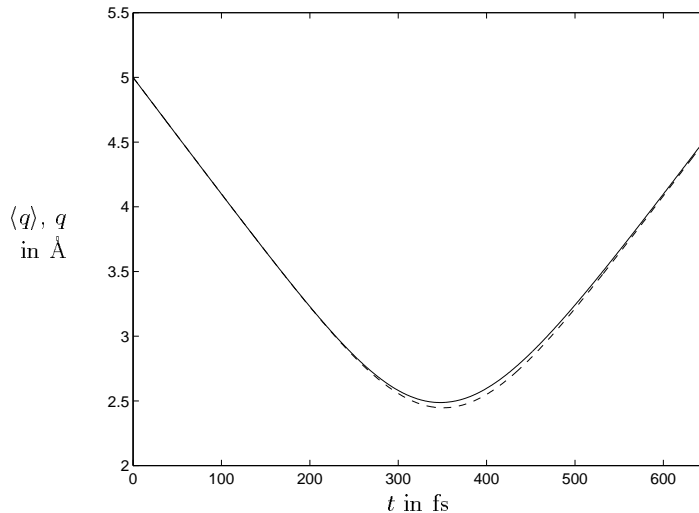
Figure 3: Results of QD- and QCMD-calculations. Shown is the position expectation \langle q \rangle (solid line) of the classical particle and its classical QCMD-trajectory q (dashed line) versus time.
