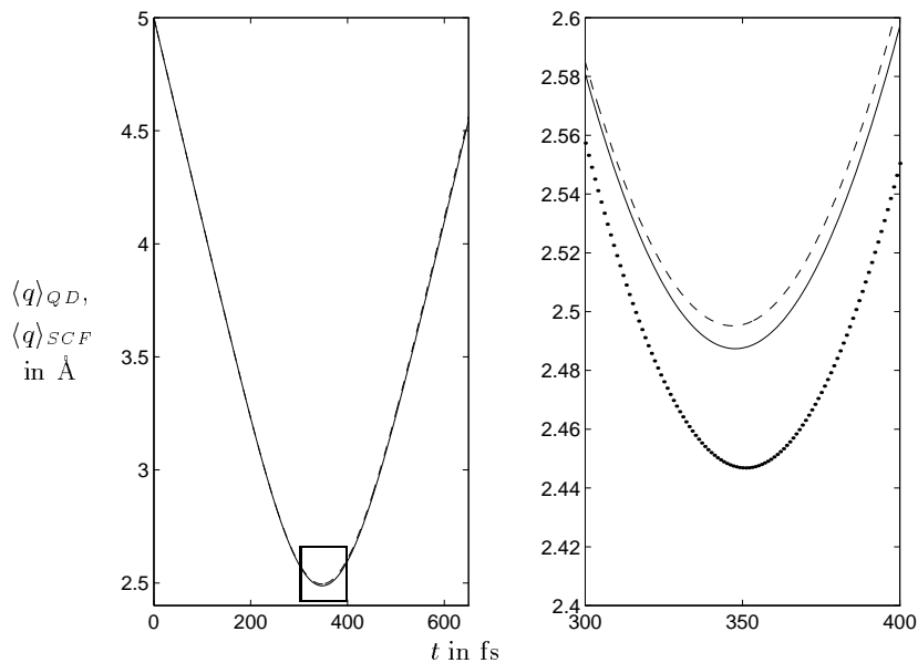
Figure 7: Results of QD- and TDSCF-calculations. The picture on the left hand side shows the corresponding position expectations \langle q \rangle_{QD} (solid line) and \langle q \rangle_{SCF} (dashed line) versus time. The region of the turning point (box) is magnified on the right hand side. Here, the additional dotted line represents the corresponding QCMD-trajectory q . Note, that this picture does not change, if we refine the stepsizes used.
