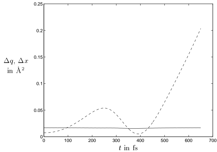
Figure 6: Evolution of variances \Delta q (dashed) and \Delta x (solid) of the full QD-wavepacket. Note the disintegration of the wavepacket in q -direction in which no attractive potential is present. It is increasing as long as the particle is moving “free” and decreasing during the collision.
