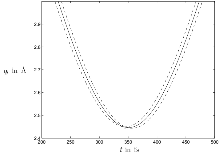
Figure 5: Crossing of different particle paths q_i in the focal point (circle). The solid line represents the QCMD-trajectory q , the dashed lines the neighboring trajectories q_{-1} and q_1 started from a slightly different initial position. Notation as explained in the text.
