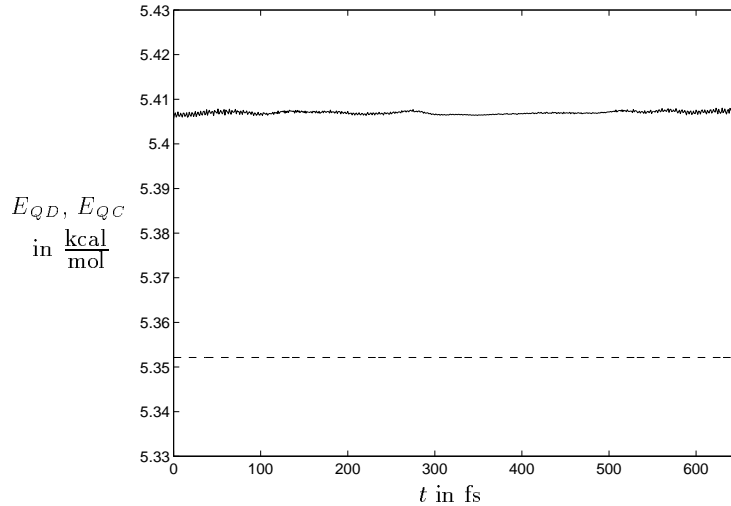
Figure 4: Conservation of energy in the QD-simulation (solid line) and the QCMD-simulation (dashed line). The difference between both values is caused by the zero-point energy \Delta E_0 = \hbar^2/8M\epsilon^2 = 0.0535 kcal/mol of the “classical” particle as discussed in Section 4.3.
