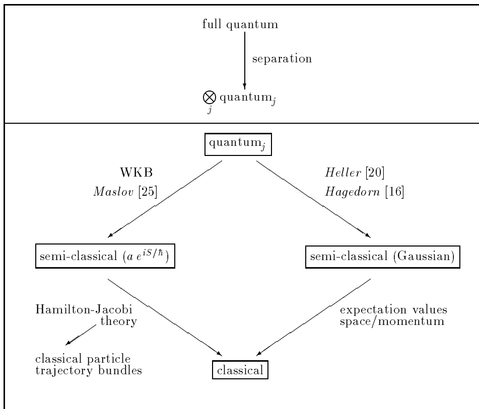
Figure 1: Different approaches to quantum-(semi-)classical models. In mixed approaches the full quantum system is first separated via the tensor product ansatz into parts j with coupled quantum description. Then, the evolution of each part j can be modeled on different levels: quantally, semi-classically, or (purely) classically. For the entire system or for each single part, the derivation of the different models from the original quantum description level can be realized, as indicated, on two different ways. On each way both steps can be justified strictly mathematically in the context of appropriate asymptotic expansions. The simultaneous justification of the separation step remains the crucial point.
