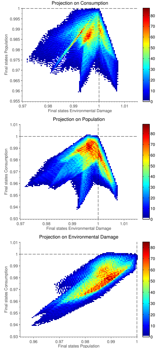
Figure 1: 2D projections of the final state vector space for 68,921 impulses in [-1, 1]^3 .
