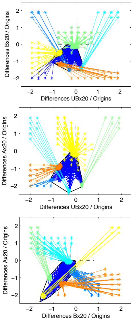
Figure 2: Clustering final state vectors from extremal scenarios.
