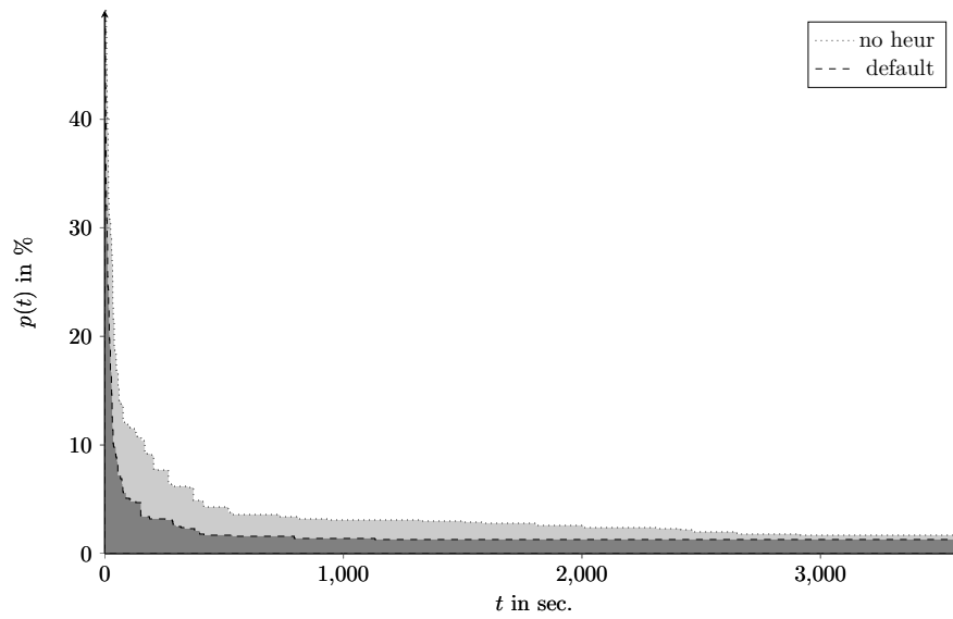
Figure 2: Course of the primal gap when running CPLEX with and without primal heuristics
