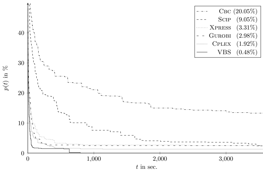
Figure 3: Course of the primal gap for five different MIP solvers plus a virtual best solver
