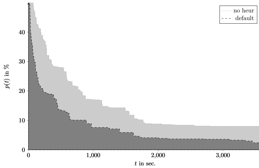
Figure 1: Course of the primal gap when running SCIP with and without primal heuristics
