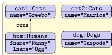
Fig. 4. An attributed graph
