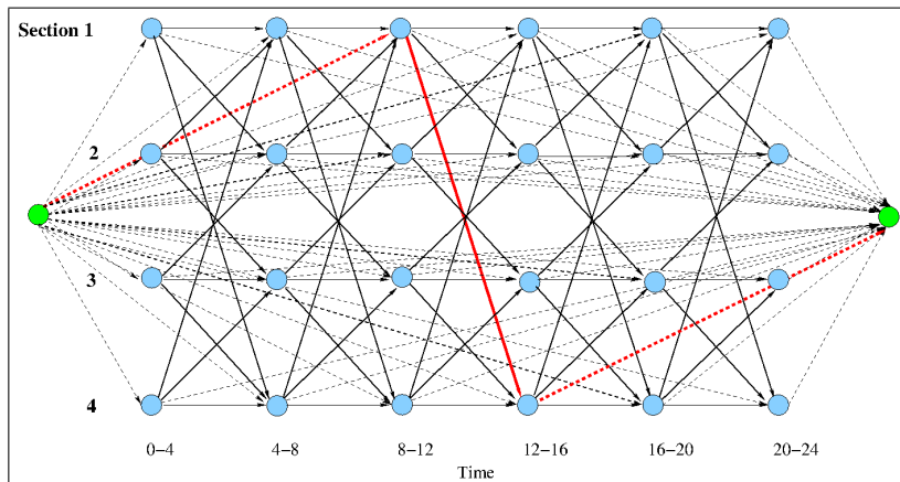
Figure 1: Construction of the tour planning graph.
