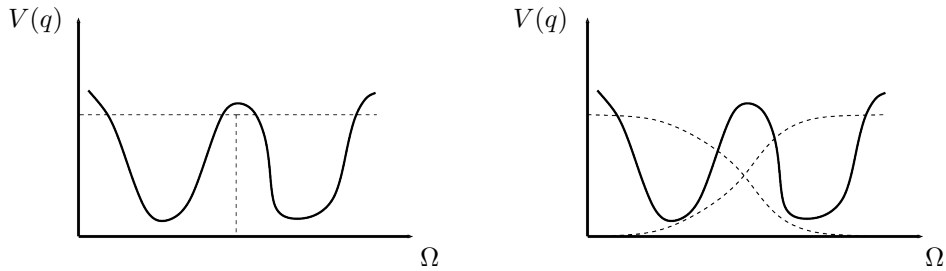
Figure 3: Left: A double wellled potential (solid line), and the hard partition of the metastable configurations (dashed line). Right: Same double wellled potential with a soft partition of metastabilities.
