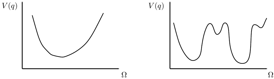
Figure 2: Left: Energy landscape of a rigid molecule with a unique minimum. Right: The energy landscape of biomolecules is in general rough, with multiple local minima.
