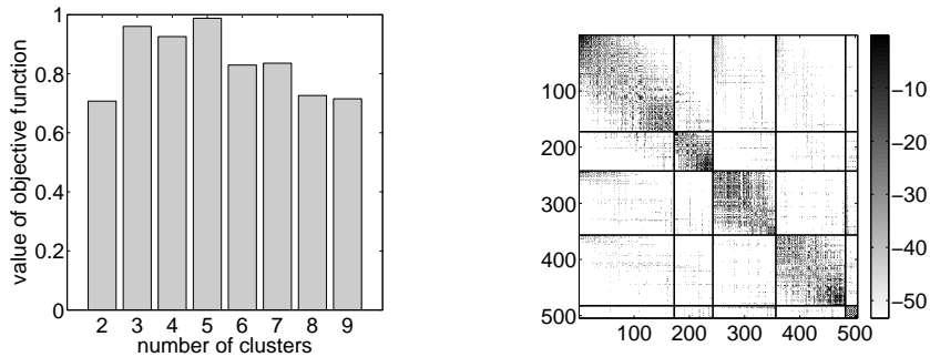
Figure 6: Left : The value of the objective function (10) for different numbers of clusters. The maximum value is achieved for n_c = 5 clusters. Right : Image of \log(P) with rows and columns resorted according to the decomposition into 5 clusters.
