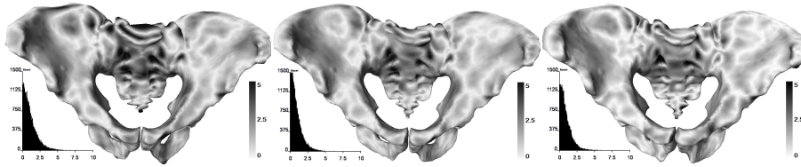
Figure 4: \mathcal{S}_T for C^0 wind Figure 5: \mathcal{S}_T for C^1 wind Figure 6: \mathcal{S}_T for C^\infty wind
