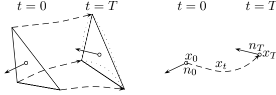
Figure 1: Usual discrete 2-current deformation (left) versus the direct approach (right)
