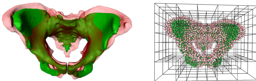
Figure 2: \mathcal{S} (dark green), \mathcal{T} (light red) Figure 3: \hat{\mathcal{S}} (green), \hat{\mathcal{T}} (red), grid
