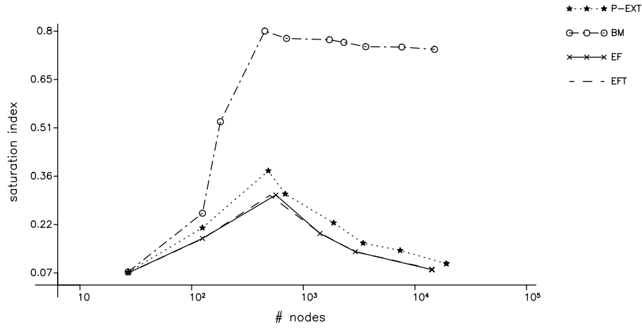
Figure 5.2: Saturation Property
