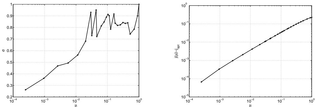
Figure 3: Left: \mu -reduction factors \sigma_k = \mu_{k+1}/\mu_k . Right: error in functional values.
