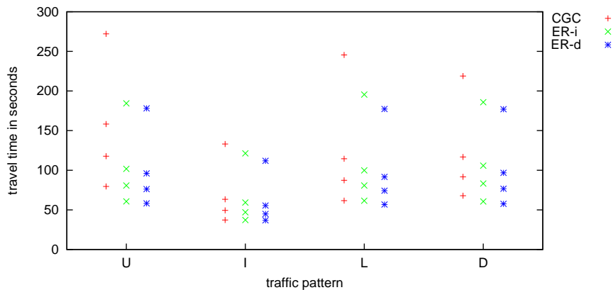
Figure 1: Simulation results for a group of four elevators in a 16-floor building.
