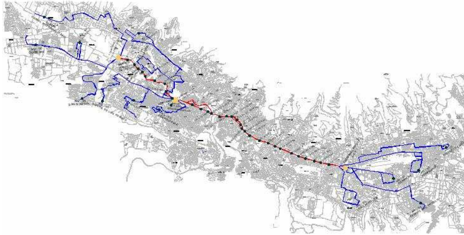
Figure 1: Trolebús system and feeder line system in Quito.
