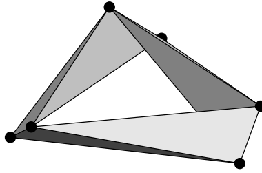
FIGURE 1.8: This partial triangulation of a twisted prism over a triangle cannot be completed to a triangulation without new vertices.
