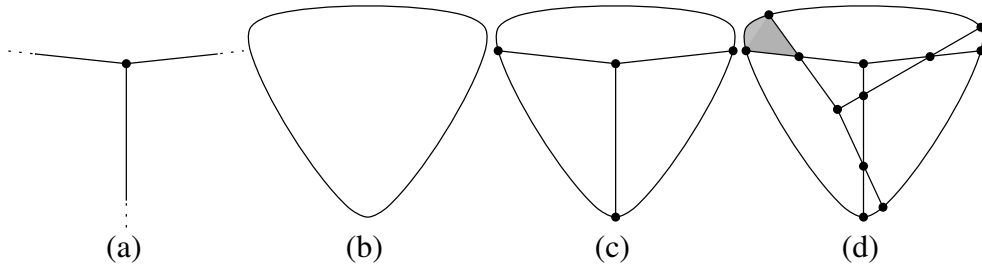
FIGURE 2.7: A part of the normal fan over the vertex \tau_{12} of Q (a), over \sigma_{123} (b), over the corresponding edge \sigma_{12} (c), and over the adjacent 2-dimensional chamber \sigma_1 (d). If \psi_{\sigma_1} is chosen in the interior of the shaded cone, and if \psi_{\sigma_2} and \psi_{\sigma_3} are chosen analogously with respect to the rotational symmetry we get the basket ball obstruction of Figure 2.6.
