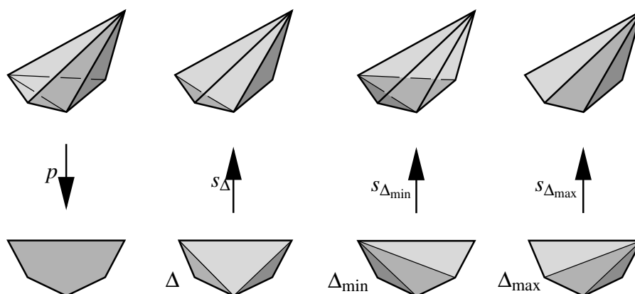
FIGURE 3.1: The canonical projection p : C(5, 3) \rightarrow C(5, 2) and characteristic sections corresponding to triangulations of C(5, 2) .
