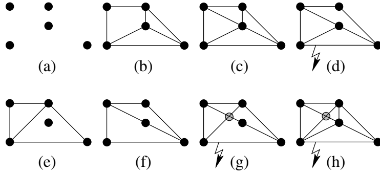
FIGURE 1.1: A planar point configuration \mathcal{A} where three of the points are collinear (a), a polyhedral subdivision (b), a triangulation (c), and a dissection of \mathcal{A} that is not a polyhedral subdivision (d); two triangulations (e) and (f) that do not use all points of \mathcal{A} , their common refinement (g) leading to a new (grey) vertex not in \mathcal{A} , and the common refinement of all triangulations of \mathcal{A} (h). Hence, (g) and (h) are polyhedral subdivisions of \text{conv}(\mathcal{A}) , but not of \mathcal{A} .
