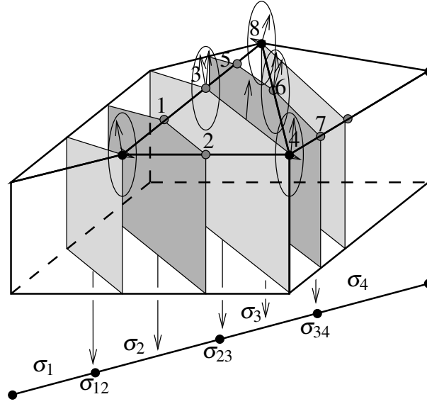
FIGURE 2.3: The pairwise cone condition.
