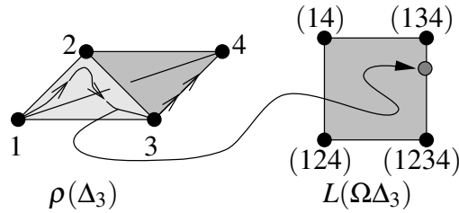
FIGURE 1.10: The string space of the 3-simplex stippled by minimal and maximal vertex. It is modelled by a 2-cube. The indicated path going first through the face \{1, 2, 3\} and then along the edge \{3, 4\} corresponds to the grey point in the relative interior of the edge \{(134), (1234)\} of the square.
