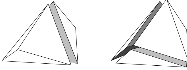
FIGURE 1.3: The two triangulations T_{Z^+} and T_{Z^-} of a set Z of 5 points in convex position in dimension 3.
