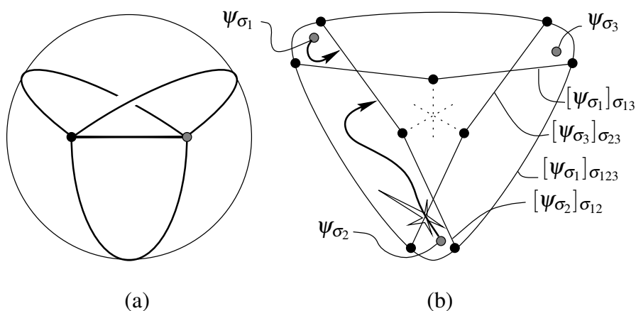
FIGURE 2.6: The “basket ball obstruction.”
