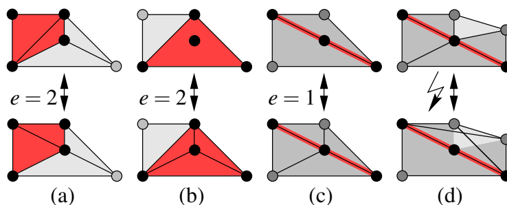
FIGURE 1.4: A bistellar operation supported (black points) on a convex quadrangle (edge flip) (a), on a triangle with an inner point (stellar operation) (b), on a line segment with an inner point (c), and an example where the link condition is not met (d).
