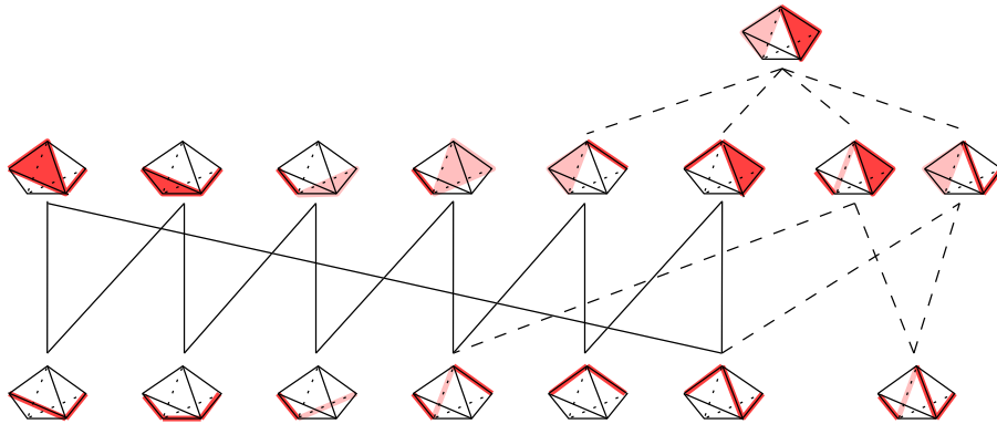
FIGURE 1.7: The poset \omega(P, \pi) where P is a bipyramid over a triangle in \mathbb{R}^3 , projecting via \pi to an interval Q in \mathbb{R} . Indicated are the inducing faces in P rather than subdivisions of Q . Note that its order complex is not homeomorphic, but homotopy-equivalent to a 1-sphere. The subposet indicated by the solid drawn covering relations is the poset \omega_{\text{coh}}(P, \pi) of all \pi -coherent subdivisions of Q , which is isomorphic to a hexagon (picture based on ZIEGLER [75, p. 297]).
