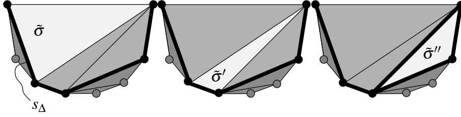
FIGURE 3.5: Finding an increasing flip in \mathcal{S}_1(8, 1) .
