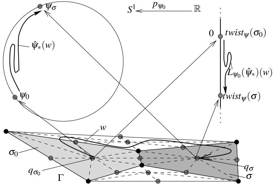
FIGURE 2.4: The twist of \sigma .
