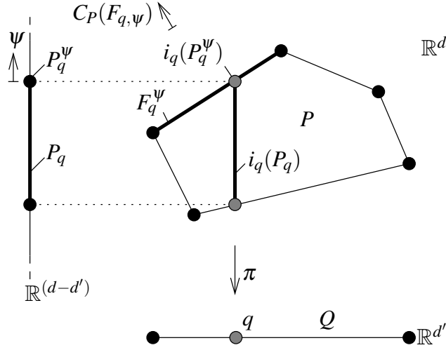
FIGURE 2.1: The face F_{q, \psi} induced by \psi \in (\mathbb{R}^{d-d'})^* .
