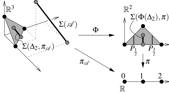
FIGURE 1.11: The secondary polytope of \{0, 1, 2\} \subset \mathbb{R} .
