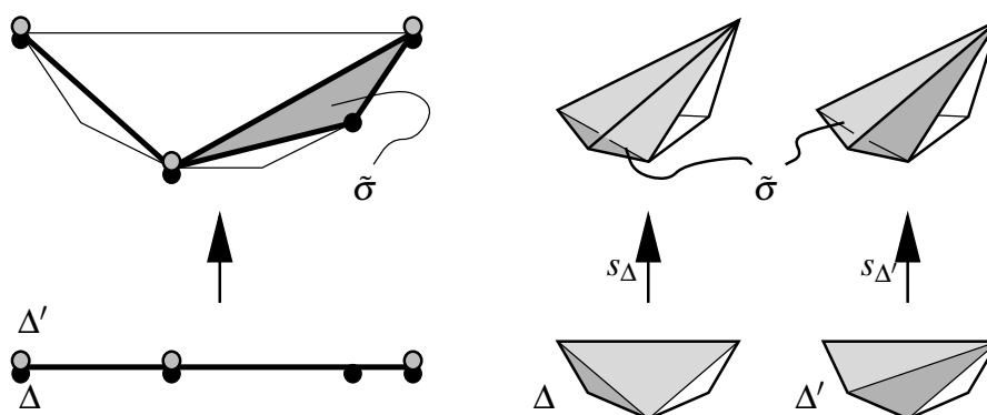
FIGURE 3.4: Increasing flips in \mathcal{S}_1(6, 1) respectively \mathcal{S}_1(5, 2) .
