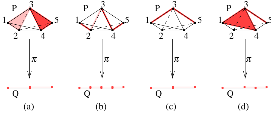
FIGURE 1.6: The induced non-tight subdivision \{123, 345\} (a), the tight induced non-coherent subdivision \{12, 23, 34, 45\} (b), the tight coherent subdivision \{13, 35\} (c), and the set of faces \{134, 35\} , which does not induce any subdivision of Q (d).
