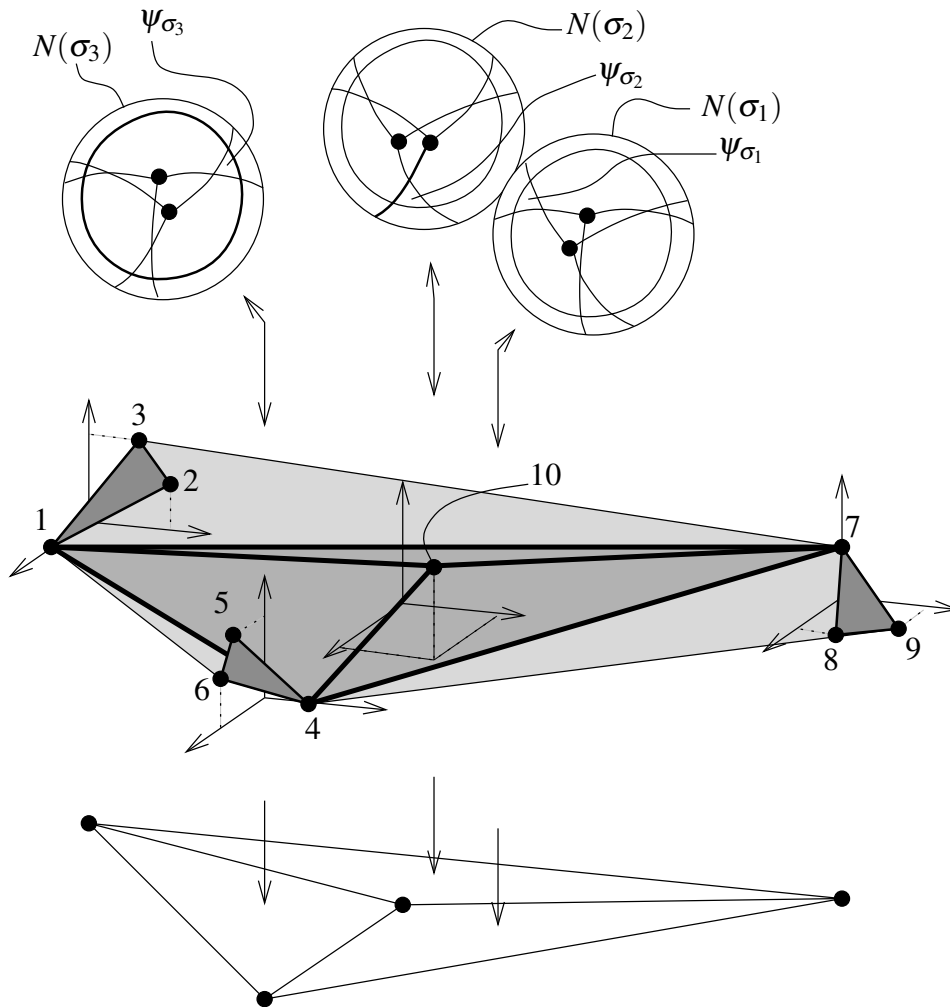
FIGURE 2.10: The medium-dark triangles correspond to the isolated locally coherent string \{(1, 4, 10), (4, 7, 10), (7, 1, 10)\} that is defined by the function values \psi_{\sigma_1} , \psi_{\sigma_2} , and \psi_{\sigma_3} for the chambers \sigma_1 , \sigma_2 , and \sigma_3 .
