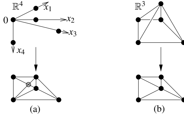
FIGURE 1.5: The chamber complexes of the projections of a 4-simplex (a) and of a 3-dimensional pyramid (b) to a planar point configuration \mathcal{A} .
