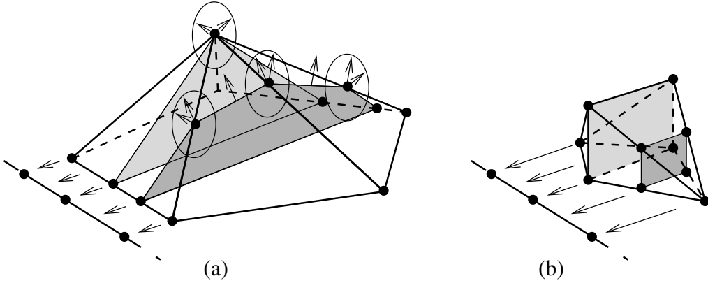
FIGURE 2.2: The normal fan relation.
