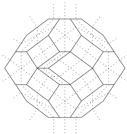
FIGURE 1.9: A zonotopal tiling corresponding to a non-realizable oriented matroid. This is indicated by the dotted “pseudolines” that form a configuration violating Pappus’ Theorem (picture from ZIEGLER [75, p. 220]).
