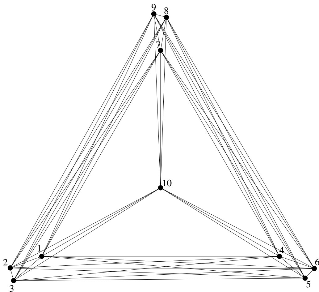
FIGURE 2.12: The chamber complex of \pi .
