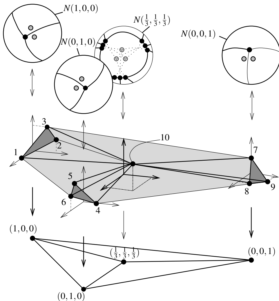
FIGURE 2.9: A sketch of \pi^{\text{deg}} : P^{\text{deg}} \rightarrow Q^{\text{deg}} : Over each vertex of Q^{\text{deg}} one perturbed basket ball is positioned. Adding the tenth vertex in the middle provides a bounding cone around the basket ball obstruction. (The grey vertices and the dotted lines are drawn to indicate the positions of the fans with respect to each other.) The 5-polytope P^{\text{deg}} is the convex hull of the three dark triangles — each of them in an \mathbb{R}^3 over one vertex of Q^{\text{deg}} — and the additional vertex (10) in the middle.
