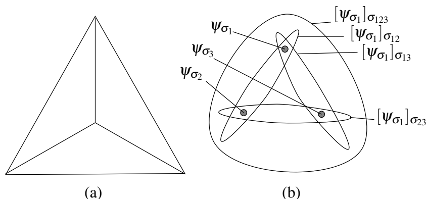
FIGURE 2.5: A simple chamber complex (a) and a sketch for a possible “locally coherent” choice of function values on this complex (b).
