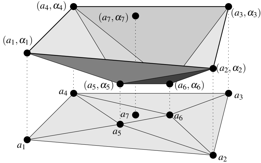
FIGURE 1.2: A regular triangulation and possible heights.
