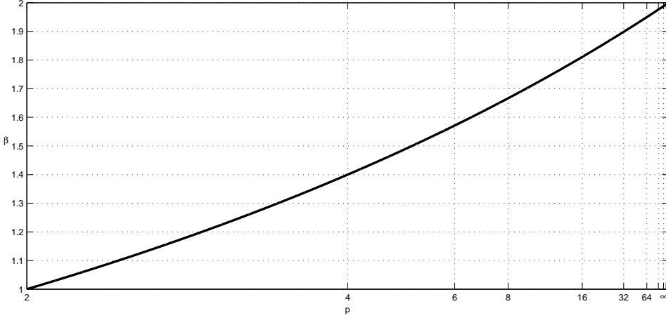
Figure 2: Convergence rates \beta according to Theorem 3.7 plotted for p \in [2, \infty] , q^{-1} + p^{-1} = 1 , and \gamma = 1 .
