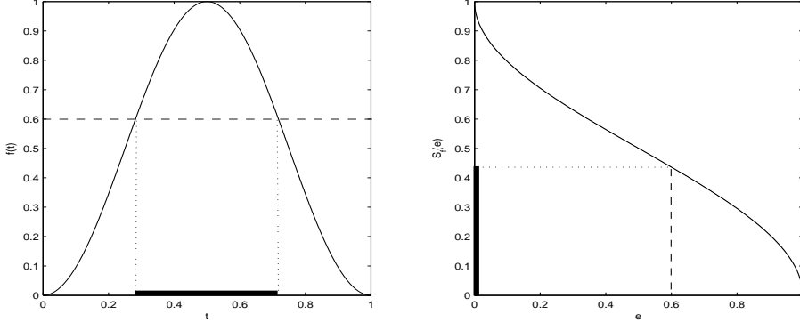
Figure 1: A function f(t) (left) and its distribution function \mathcal{S}_f(e) (right). The value of the distribution function at e is given by the area on which f is above e .
