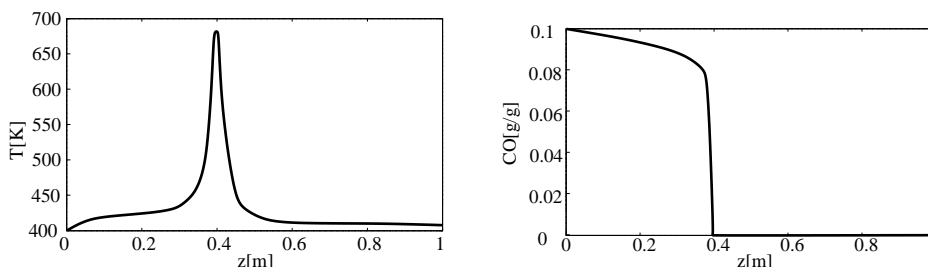
Figure 1: Reactor runaway (temperature and CO concentration)
