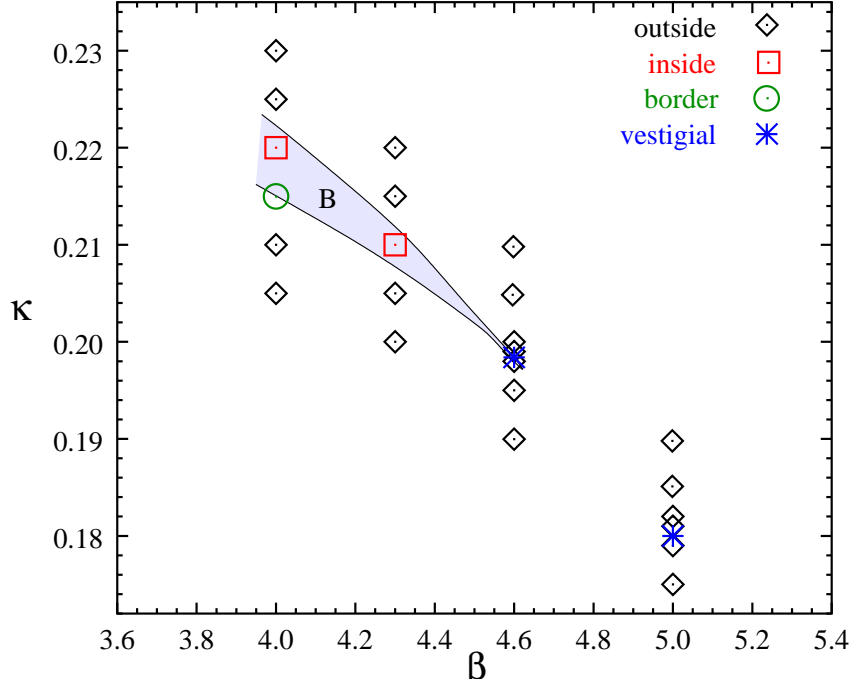
FIG. 5: The part of the phase diagram studied in this work. Squares denote (\beta, \kappa) -pairs where a finite value of \langle \bar{\psi} i \gamma_5 \tau^3 \psi \rangle_{h=0} is found. Diamonds refer to points where \langle \bar{\psi} i \gamma_5 \tau^3 \psi \rangle_{h=0} = 0 . Stars denote points where a finite value of \langle \bar{\psi} i \gamma_5 \tau^3 \psi \rangle_{h=0} is uncertain. The lines indicate the position of the critical lines \kappa_c^{(1)}(\beta) and \kappa_c^{(2)}(\beta) . The shaded region labeled B refers to the parity-flavor breaking phase. The point (\beta, \kappa) = (4.0, 0.215) seems to lie very close to the border of the broken phase.
