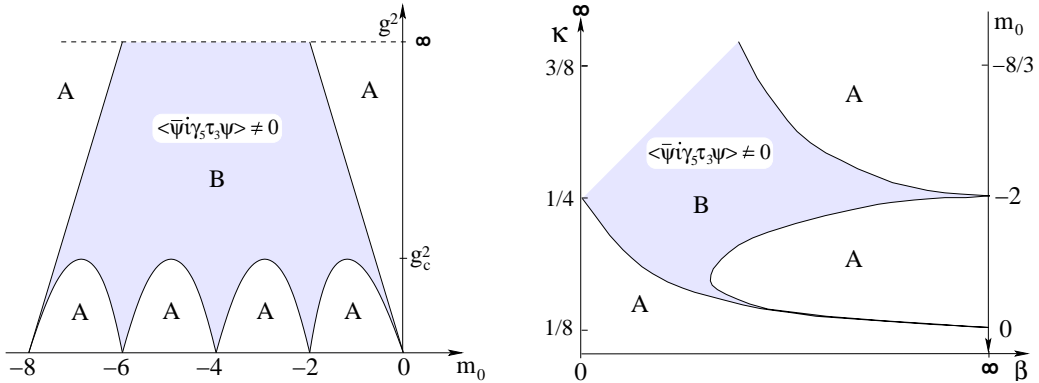
FIG. 1: The phase diagram proposed by Aoki et al. in the (g^2, m_0) -plane (left hand side) and in the (\beta, \kappa) -plane (right hand side). The shaded region labeled B denotes the phase where flavor and parity are spontaneously broken. Both symmetries are conserved in regions labeled A .
