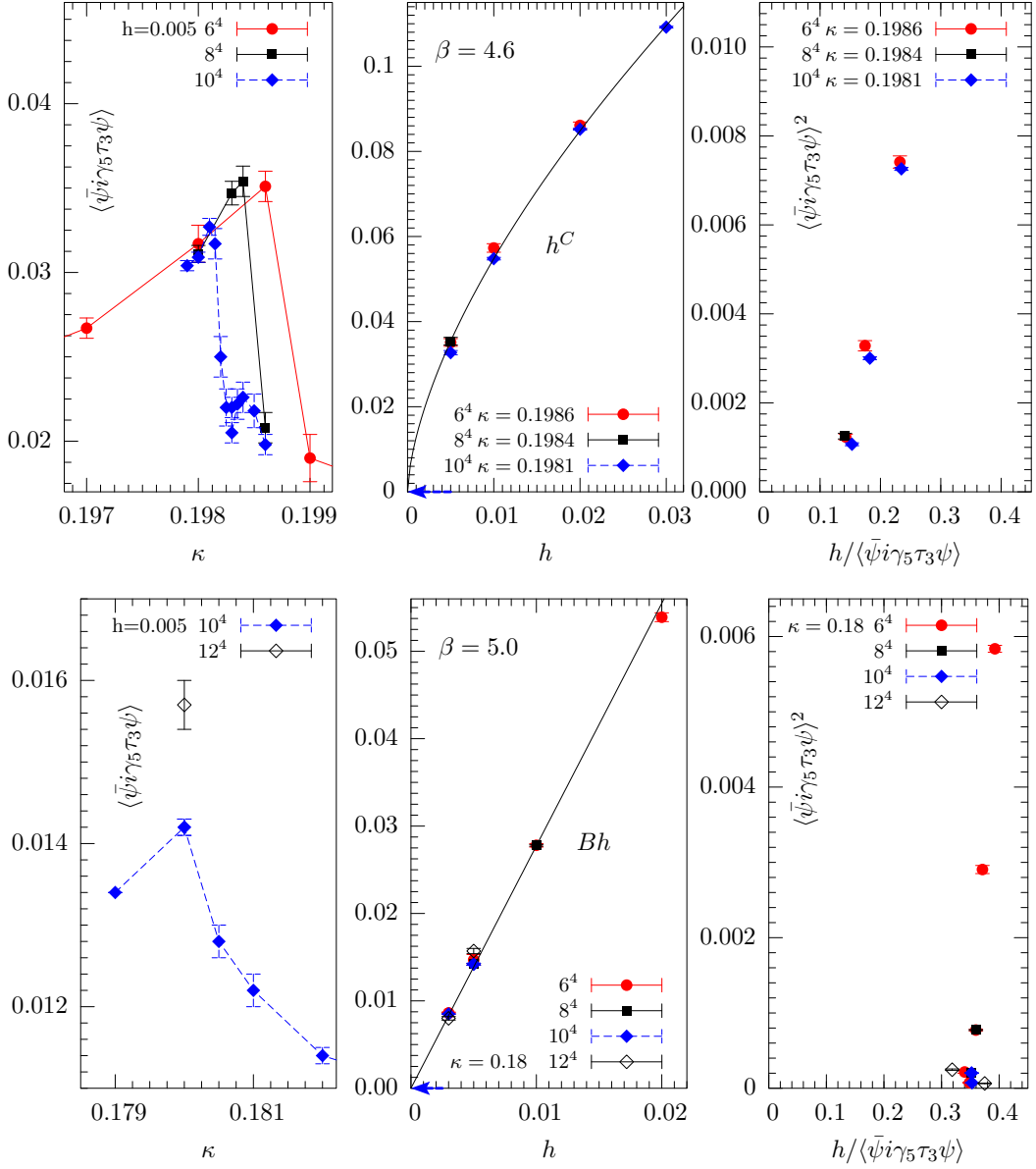
FIG. 4: In the left column data for \langle \bar{\psi} i \gamma_5 \tau_3 \psi \rangle from lattices of various sizes are shown as a function of \kappa at h = 0.005 fixed (the lines are drawn to guide the eye). The extrapolation to h = 0 in the infinite volume limit is shown in the center column. In the right column the corresponding Fisher plots are shown. The upper row contains data at \beta = 4.6 from lattices of sizes 6^4 , 8^4 and 10^4 . The lower row shows measurements for \beta = 5.0 from lattices of sizes 10^4 and 12^4 .
