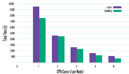
Application Benchmark TURBOMOLE Lustre versus Cray DataWarp
