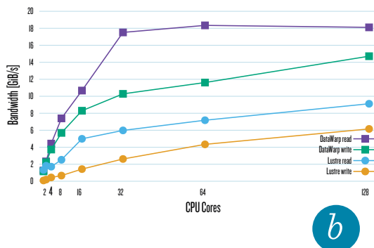
Synthetic IOR Benchmark Lustre versus Cray DataWarp
