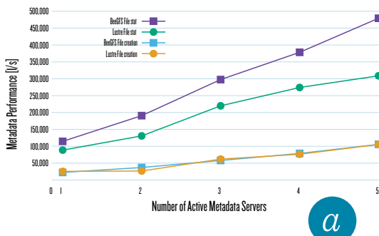
Scaling of Metadata Performance on I/O Test Bed
