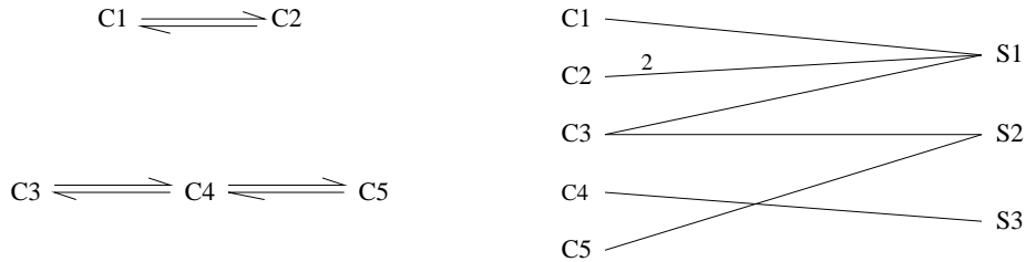
Figure 8: Example of a chemical reaction network by Feinberg due to Edelstein.
