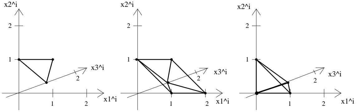
Figure 9: Newton Polytopes of system by Edelstein.
