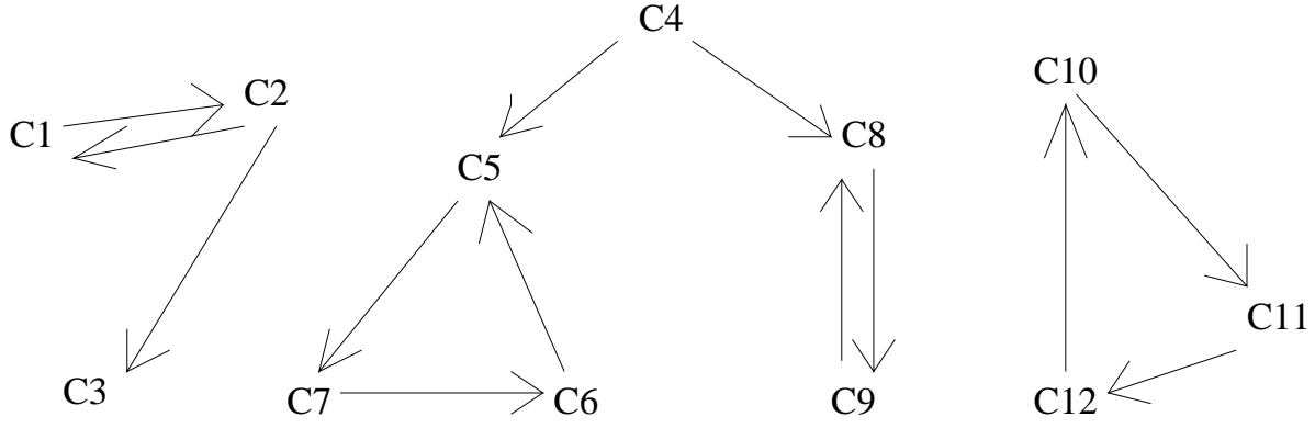
Figure 3: A reaction network with three connected components (linkage classes), four terminal strong linkage classes and two strong linkage classes which are not terminal.
