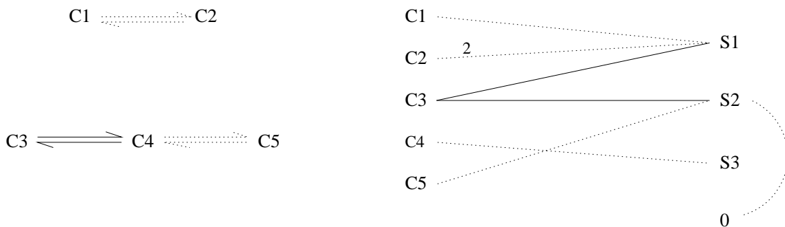
Figure 11: Parts of the directed graph of the example by Edelstein which corresponds to the alternating cell which is responsible for the positive solution.
