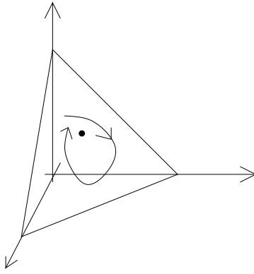
Figure 2: A trajectory within an affine subspace.
