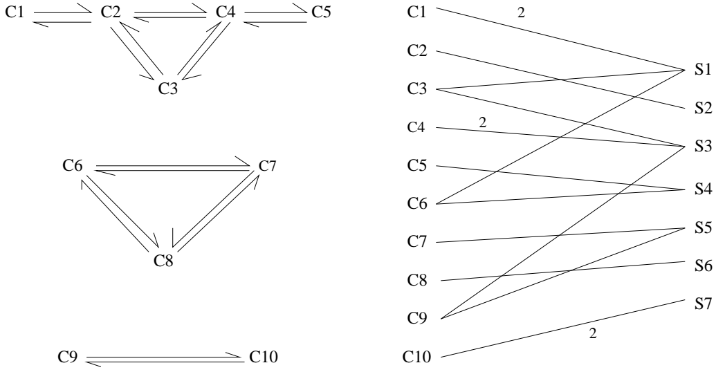
Figure 7: Example by Feinberg illustrating the assumptions in the Deciciency One Theorem.
