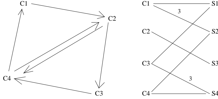
Figure 5: A Simple cycle with four complexes.
