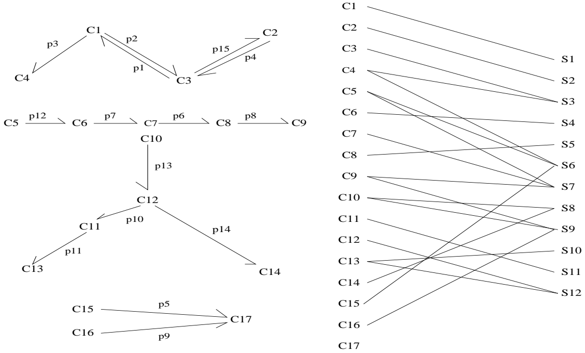
Figure 6: Enzyme synthesis in a bacteriell cell (Heinmets).
