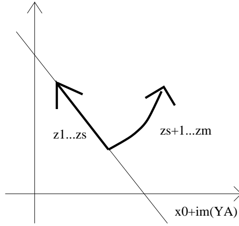
Figure 4: Nonlinear parametrization derived from Smith normal form.
