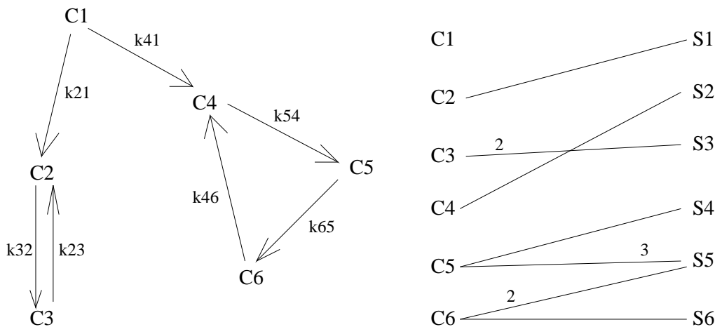
Figure 1: A reaction network with six complexes as a weighted directed graph and a weighted bipartite graph for the composition of complexes as sums of species.
