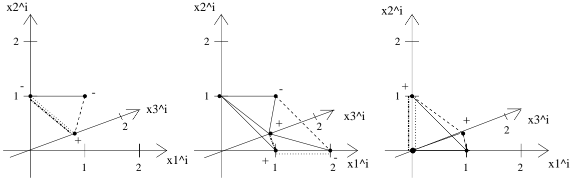
Figure 10: Mixed subdivision of Newton Polytopes of system by Edelstein.
