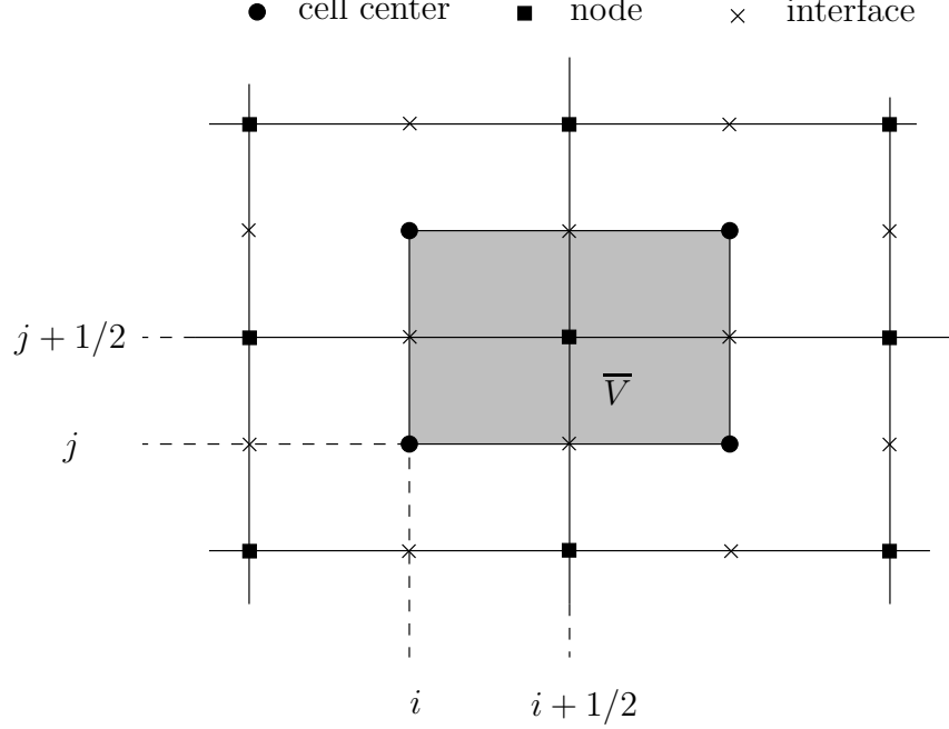
FIGURE 12. Two dimensional Cartesian grid.
