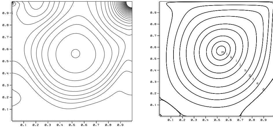
FIGURE 6. Driven cavity at Re = 1000 , 128 \times 128 grid cells: 30 contour lines of the nodal pressure p_v^{(2)} in [-0.4, 0.4] (left) and streamlines (right). Streamline values and labels are taken from [29].
