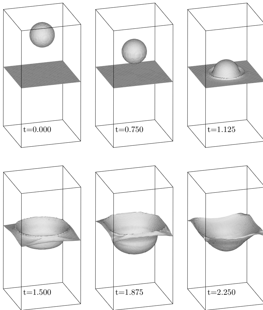
FIGURE 11. Three-dimensional falling “droplet” at Fr = 1 and density ratio 1000: Iso-surface \rho = 500 of density.
