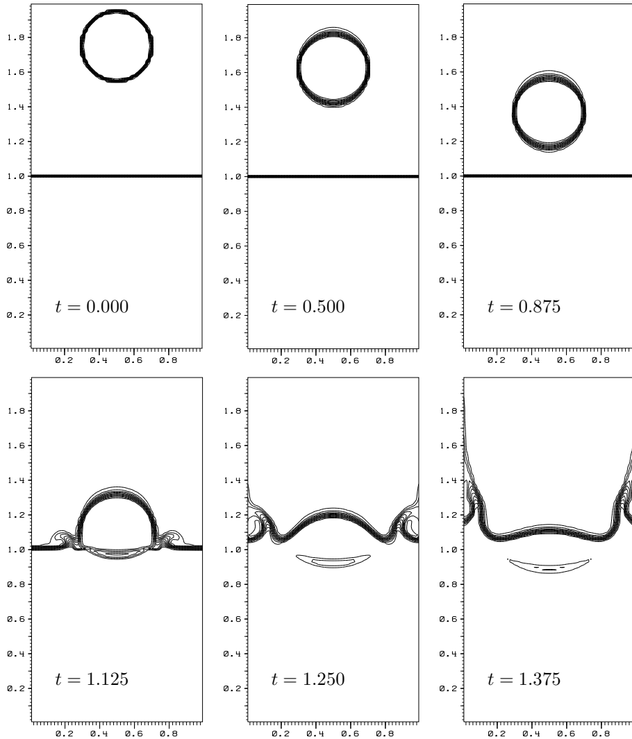
FIGURE 9. Two-dimensional falling “droplet” at Fr = 1 and density ratio 1000: Contour lines of density in [1,1000] .
