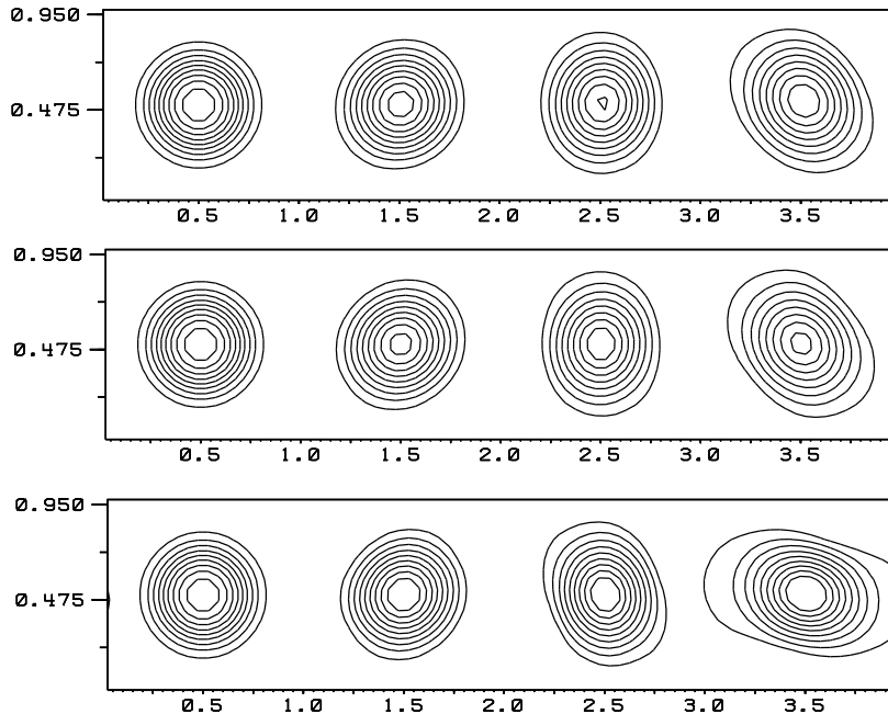
FIGURE 2. Advection of a vortex at times t = 0.0, 1.0, 2.0, 3.0 : 9 contour lines of the stream-function in [0.02, 0.18] . Unlimited slopes (top), monotonized central-difference (middle) and Sweby's limiter with k := 1.8 (bottom).
