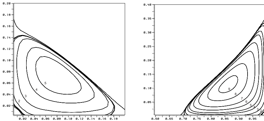
FIGURE 7. Driven cavity at Re=1000 , 128 \times 128 grid cells: streamlines in the left and right bottom secondary vortices. Values and labels are taken from [29].
