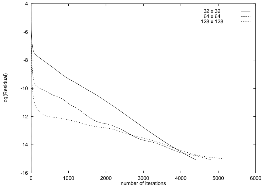
FIGURE 5. Driven cavity at Re = 1000 : Residual versus number of iterations for 32 \times 32 , 64 \times 64 and 128 \times 128 grid cells computations; coarser grid solutions have been taken as initial data for finer grid solutions.
