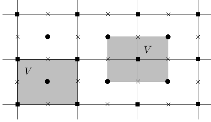
FIGURE 1. Cell ( V ) and node centered ( \bar{V} ) control volumes; cell centers, nodes and the midpoints of the interfaces are marked by circles, squares and crosses, respectively
