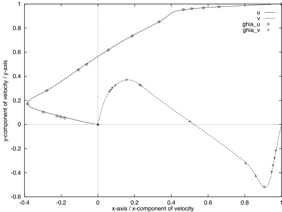
FIGURE 8. Driven cavity at Re=1000 , 128 \times 128 grid cells: horizontal (vertical) component of the velocity along the vertical (horizontal) line through the geometric center of the cavity; present results (solid line) and reference solution from [29] (dots).
