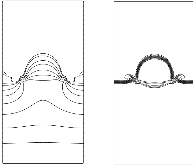
FIGURE 10. Two-dimensional falling “droplet” at Fr = 1 and density ratio 1000: 10 contour lines of the cell interface pressure p_x^{(2)} at -999, -990, -900, -800, -600, -400, -200, 0, 200 and 400 (left) and 10 contour lines of the density in [1, 1000] (right) at t = 1.125 .
