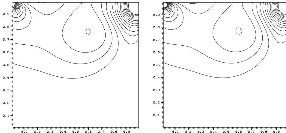
FIGURE 3. Driven cavity at Re = 100 , C = 0.8 : 30 contour lines of the nodal pressure p_{\nabla}^{(2)} in [-0.4, 0.4] . 64 \times 64 (left) and 256 \times 256 (right) grid cells.
