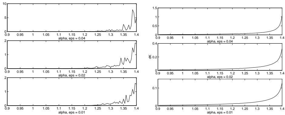
(a) Model problem with a = 2 and b = 1 .
